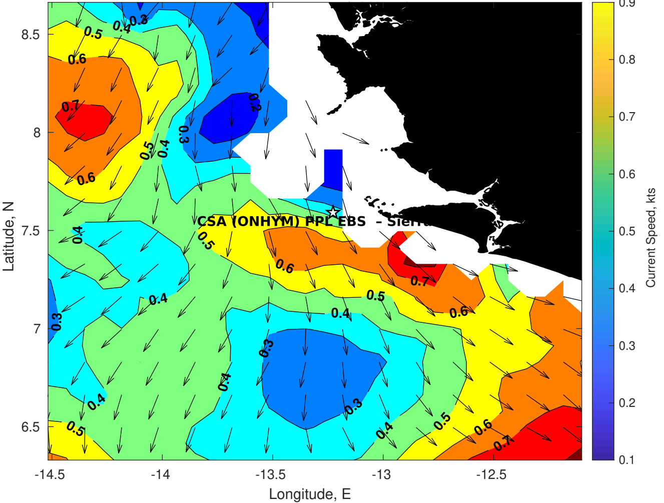
Surface Currents for CSA (ONHYM) PPL EBS - Sierra Leone at 08-Dec-2025 00:00:00
