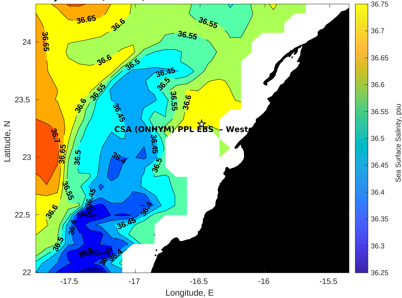
Surface Salinity for CSA (ONHYM) PPL EBS - Western Sahara at 08-Dec-2025 00:00:00
