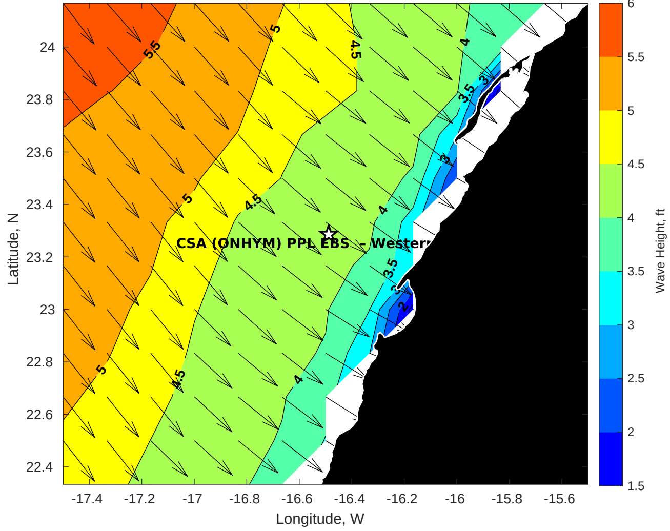
GFS Wave Height (ft) for CSA (ONHYM) PPL EBS - Western Sahara at 08-Dec-2025 21:00:00
