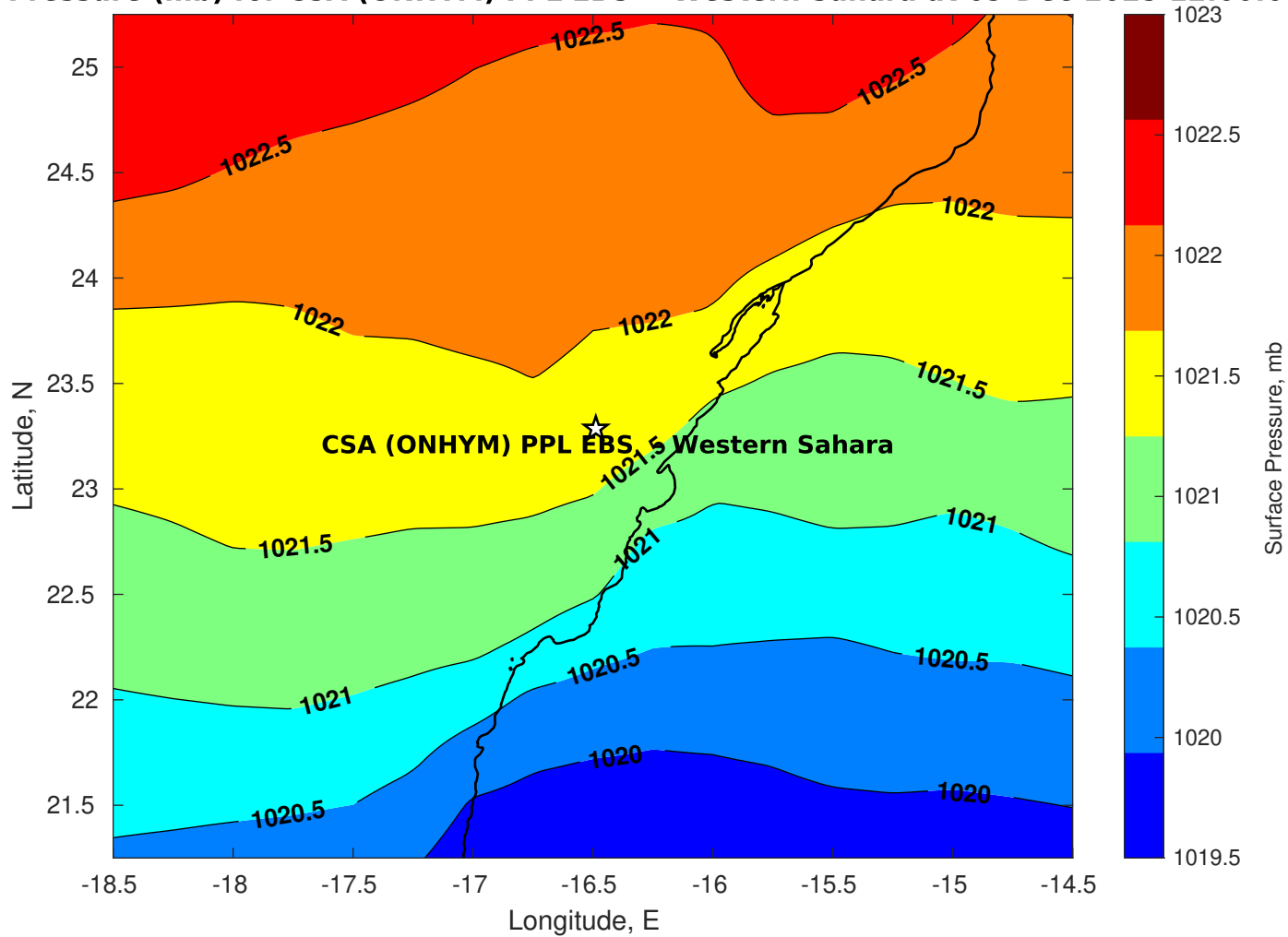
Surface Pressure (mb) for CSA (ONHYM) PPL EBS - Western Sahara at 09-Dec-2025 12:00:00
