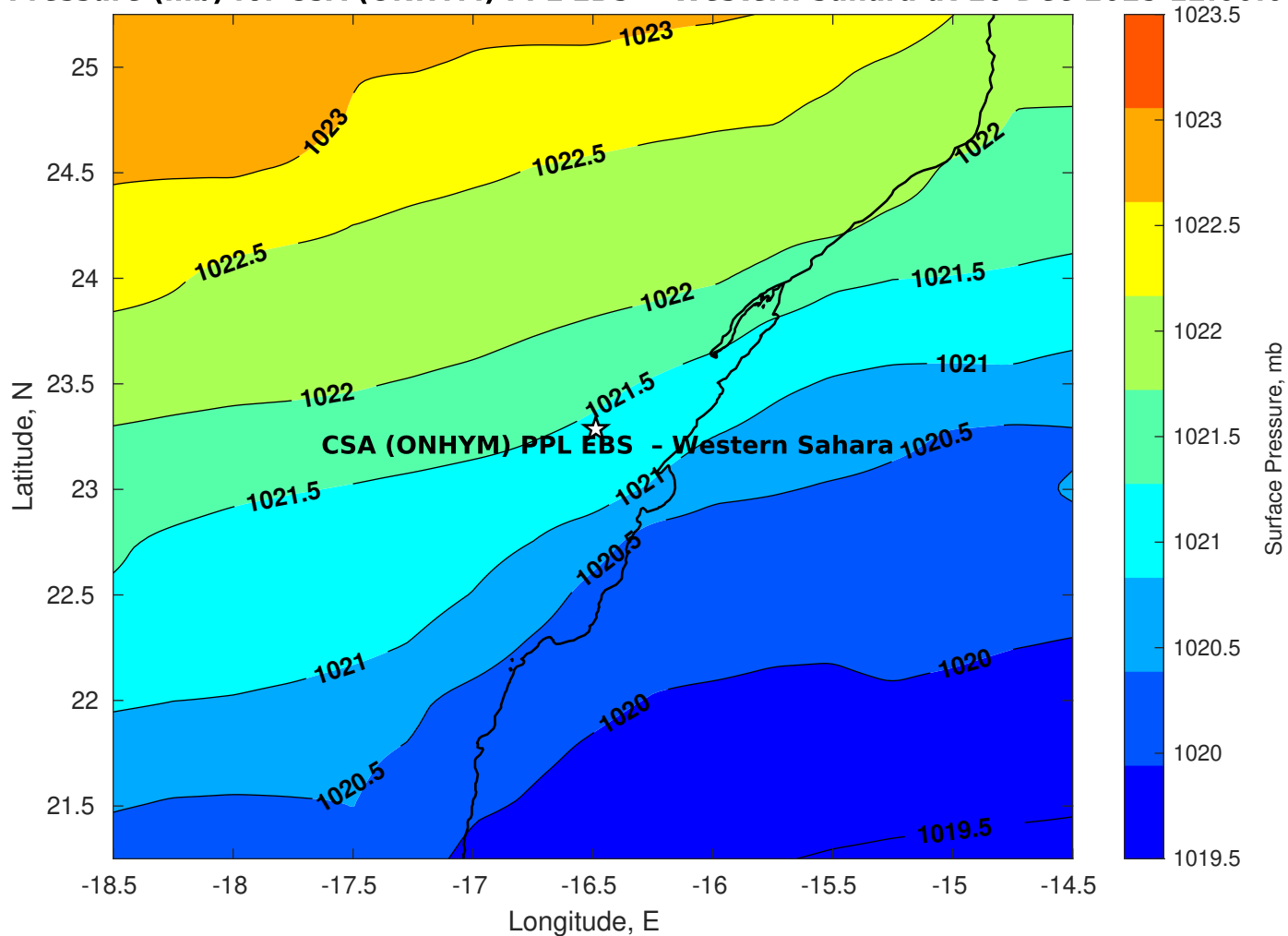
Surface Pressure (mb) for CSA (ONHYM) PPL EBS - Western Sahara at 10-Dec-2025 12:00:00
