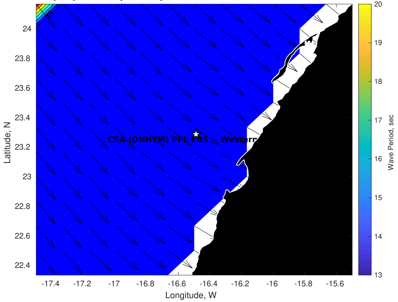
GFS Wave Period (sec) for CSA (ONHYM) PPL EBS - Western Sahara at 08-Dec-2025 21:00:00
