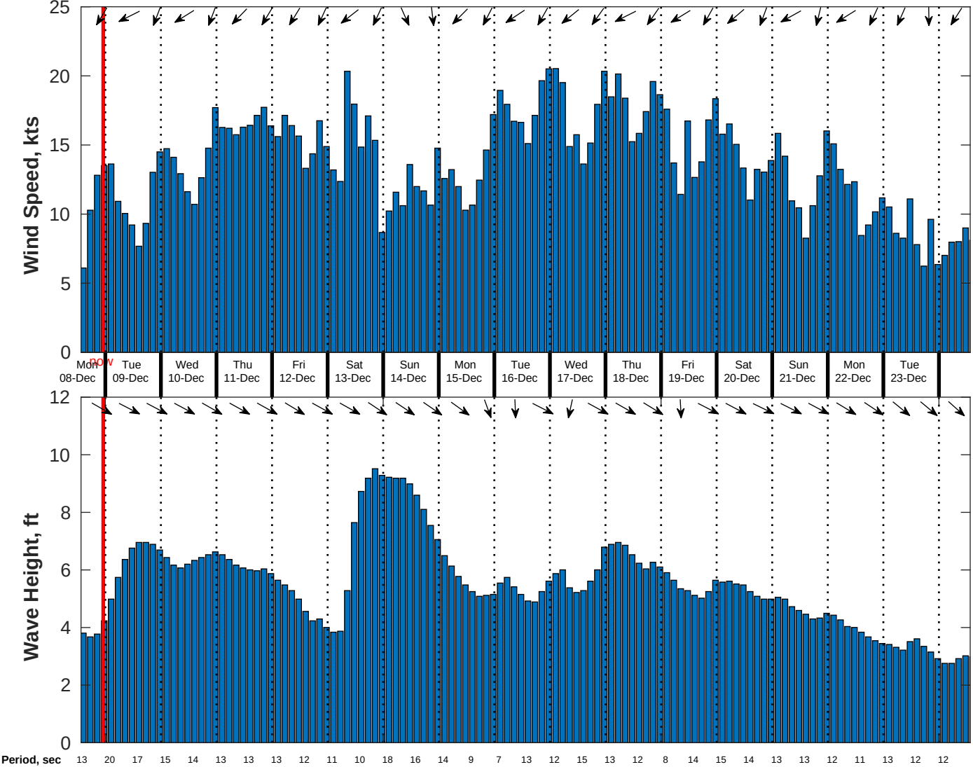
Wind & Wave Forecast for CSA (ONHYM) PPL EBS - Western Sahara from 08-Dec-2025 13:00:00 to 24-Dec-2025 13:00:00
