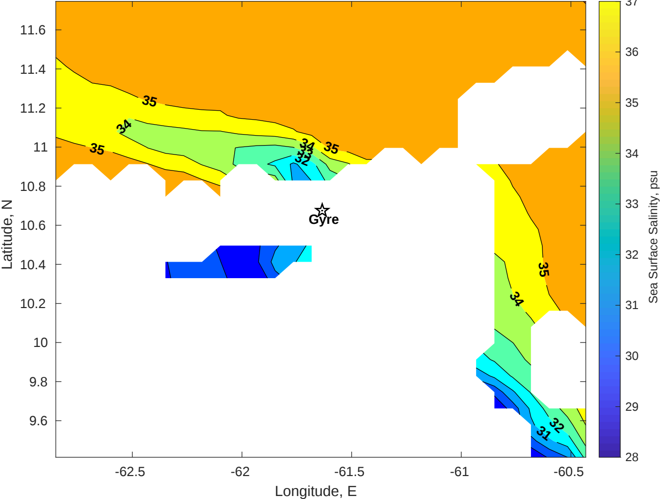
Surface Salinity for Gyre at 08-Dec-2025 00:00:00
