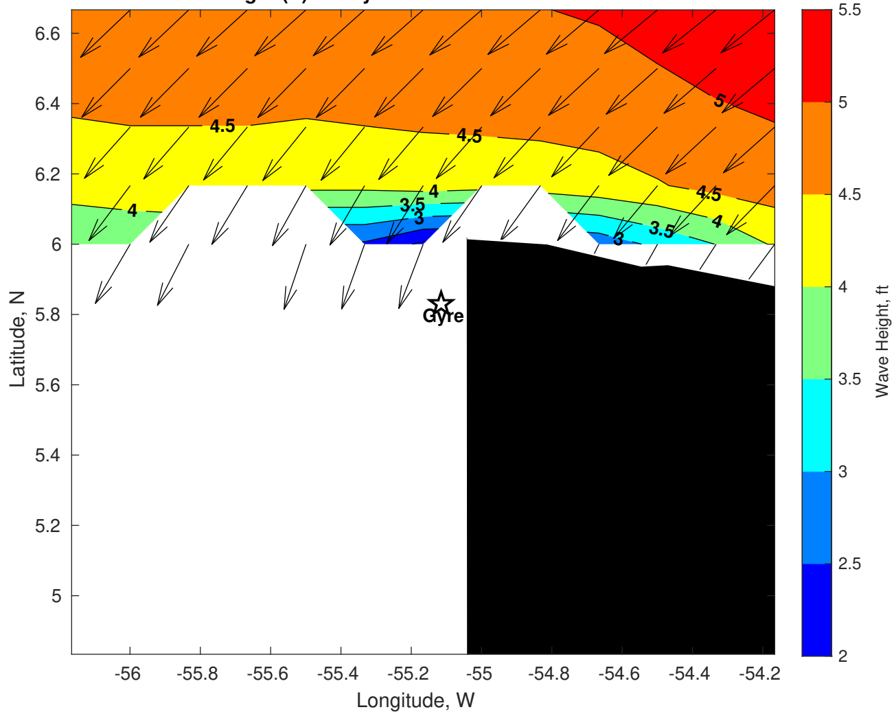
GFS Wave Height (ft) for Gyre at 06-Dec-2025 21:00:00
