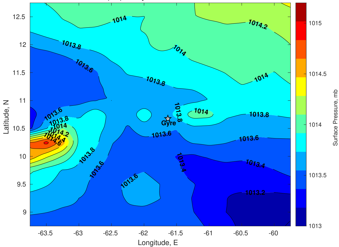
Surface Pressure (mb) for Gyre at 10-Dec-2025 12:00:00
