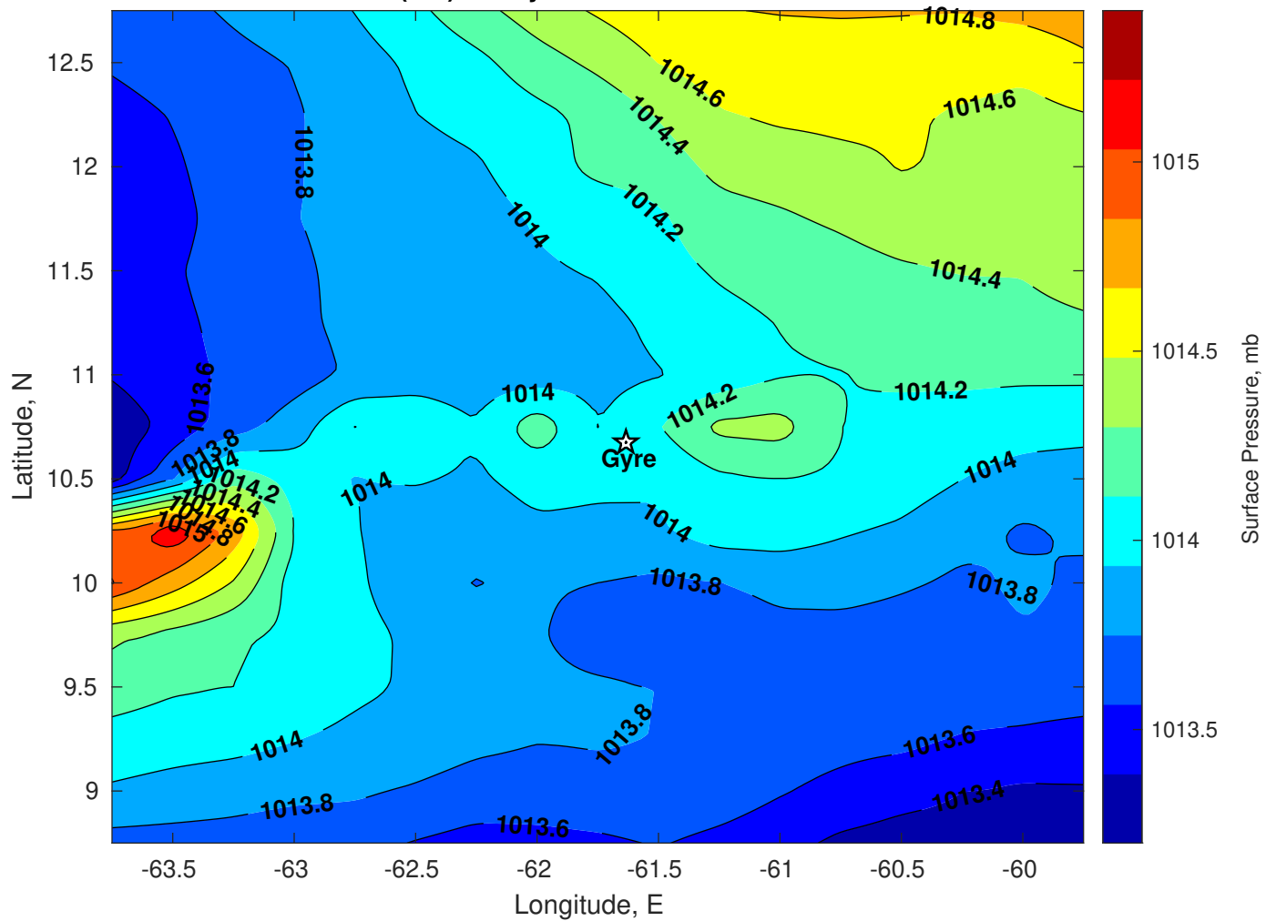
Surface Pressure (mb) for Gyre at 09-Dec-2025 12:00:00
