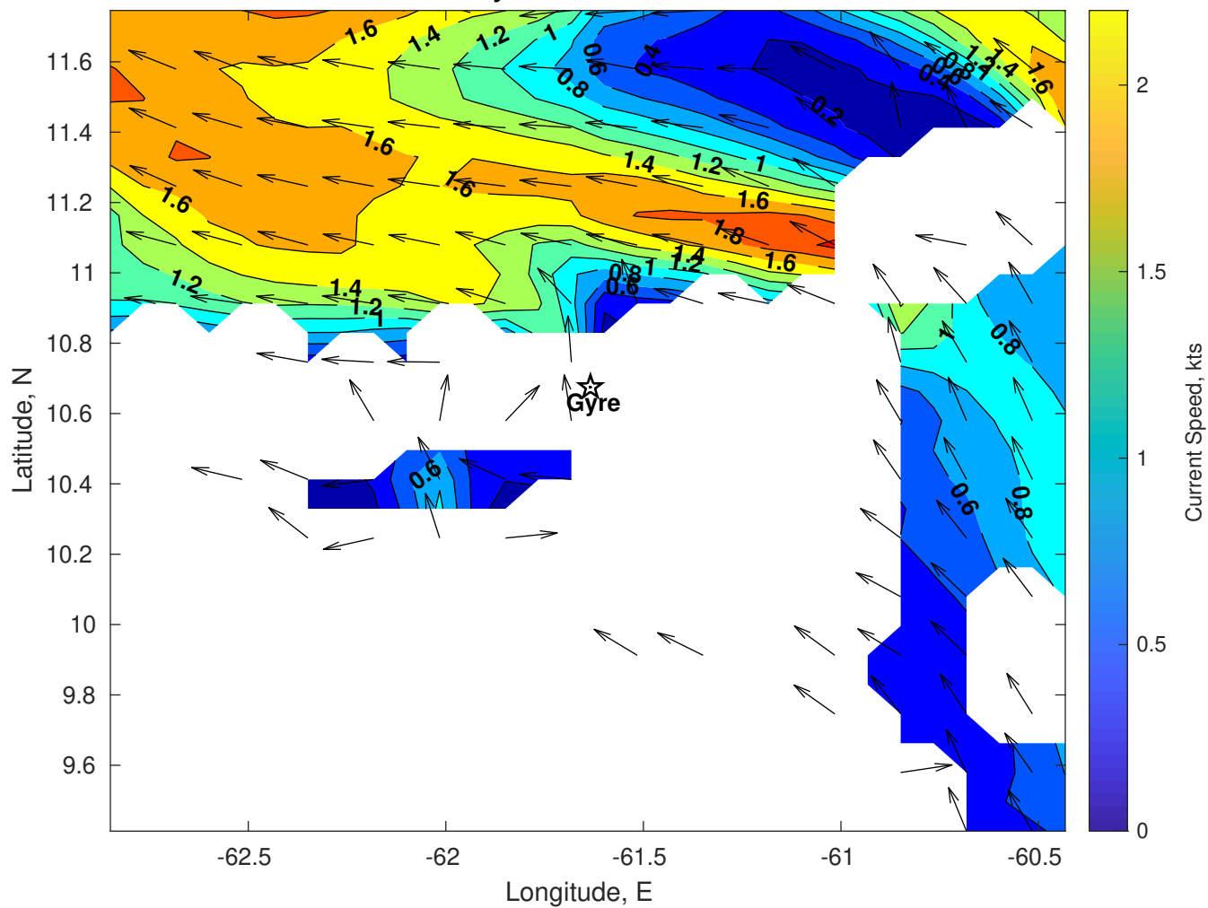
Surface Currents for Gyre at 08-Dec-2025 00:00:00
