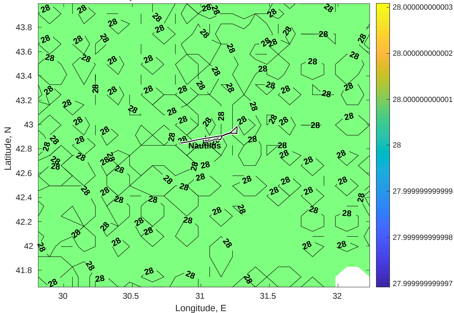
Surface Salinity for Nautilus at 08-Dec-2025 00:00:00
