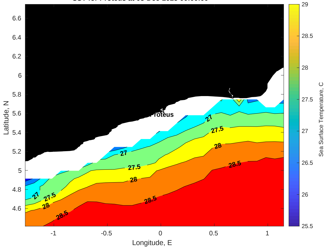
SST for Proteus at 08-Dec-2025 00:00:00
