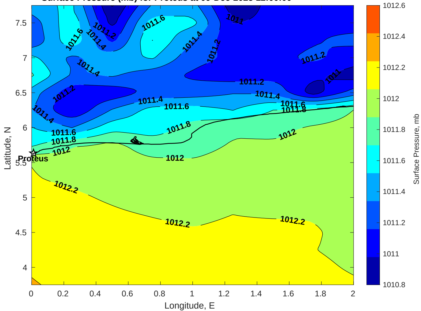
Surface Pressure (mb) for Proteus at 09-Dec-2025 12:00:00
