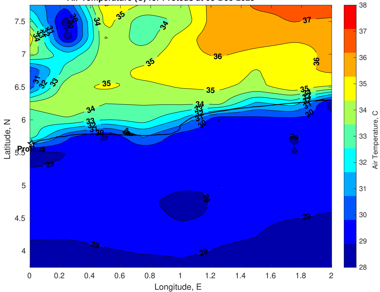
Air Temperature (C) for Proteus at 08-Dec-2025
