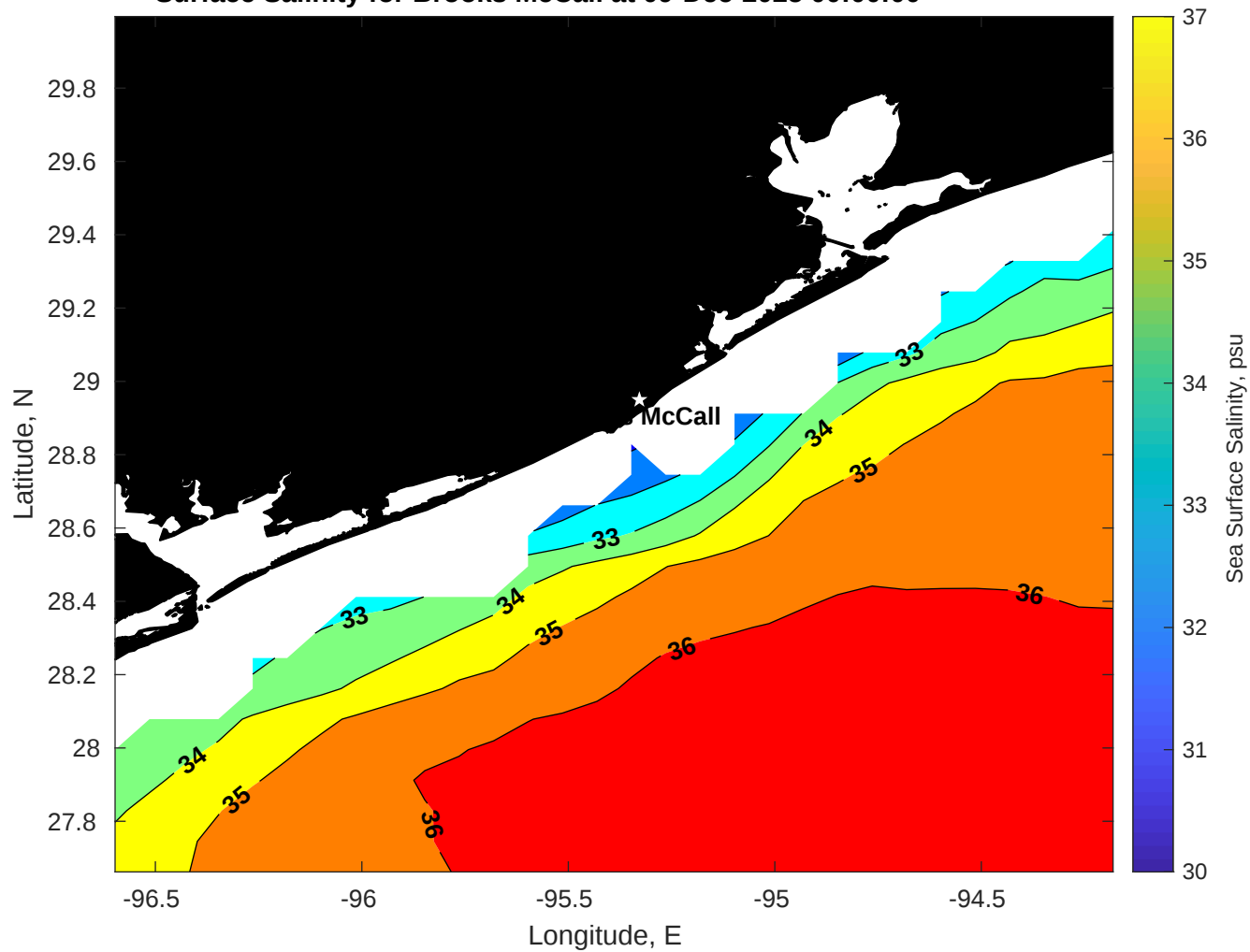
Surface Salinity for Brooks McCall at 09-Dec-2025 00:00:00
