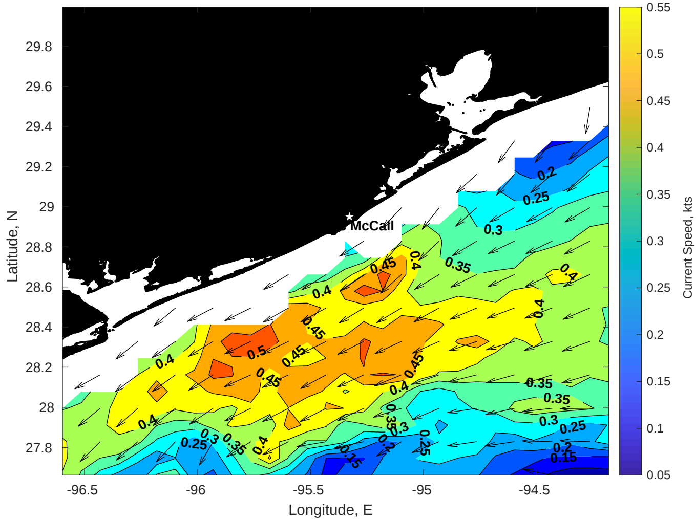
Surface Currents for Brooks McCall at 09-Dec-2025 00:00:00
