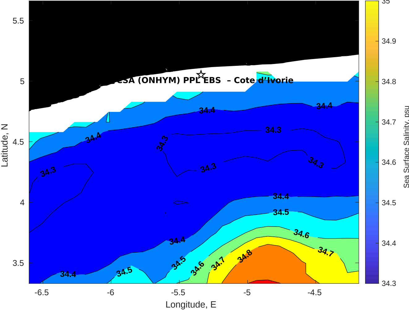
Surface Salinity for CSA (ONHYM) PPL EBS - Cote d'Ivoire at 09-Dec-2025 00:00:00
