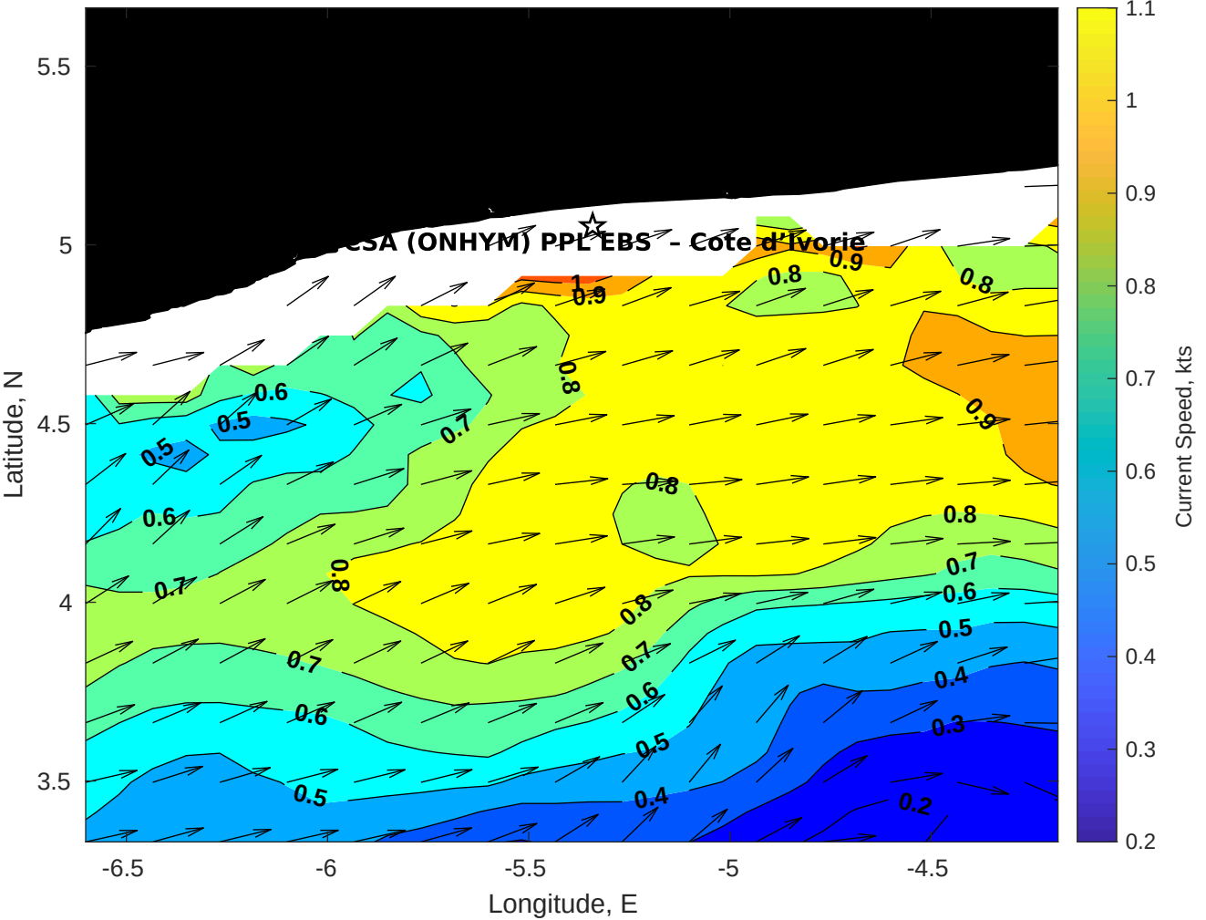
Surface Currents for CSA (ONHYM) PPL EBS - Cote d'Ivoire at 09-Dec-2025 00:00:00
