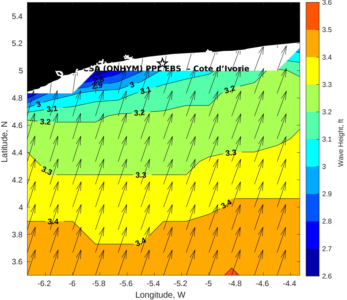
GFS Wave Height (ft) for CSA (ONHYM) PPL EBS - Cote d'Ivoire at 10-Dec-2025 09:00:00
