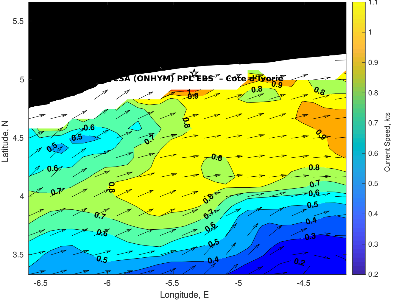
Surface Currents for CSA (ONHYM) PPL EBS - Cote d'Ivoire at 09-Dec-2025 00:00:00
