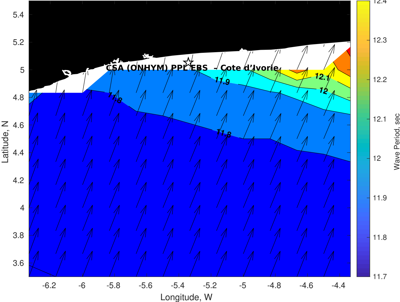
GFS Wave Period (sec) for CSA (ONHYM) PPL EBS - Cote d'Ivoire at 10-Dec-2025 09:00:00
