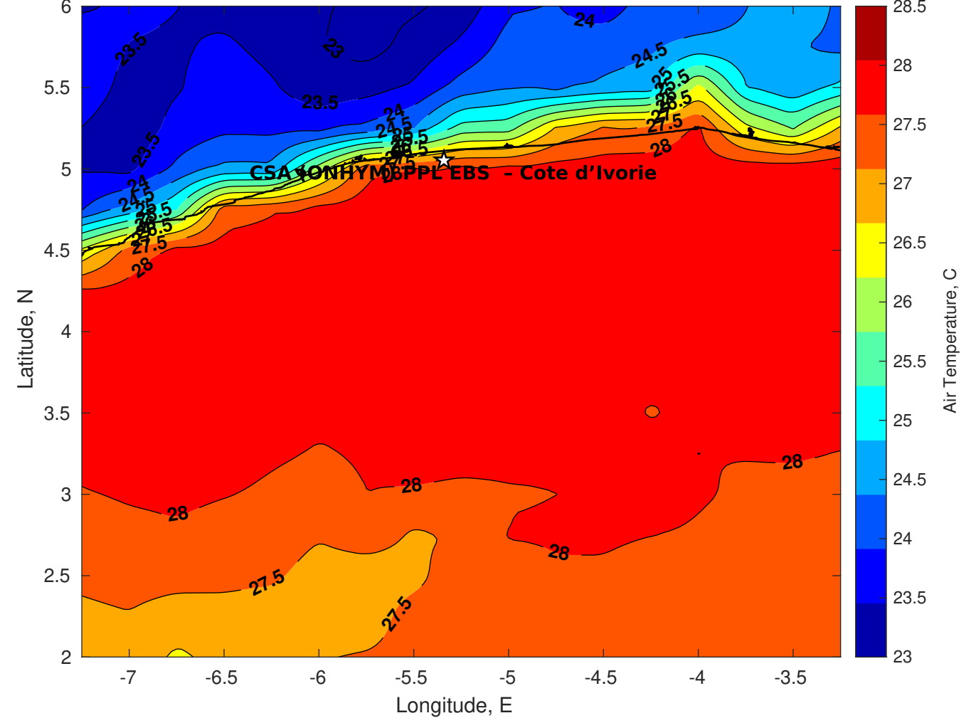
Air Temperature (C) for CSA (ONHYM) PPL EBS - Cote d'Ivoire at 10-Dec-2025
