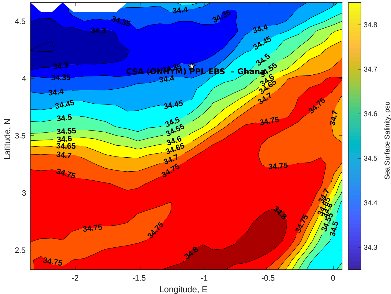
Surface Salinity for CSA (ONHYM) PPL EBS - Ghana at 09-Dec-2025 00:00:00
