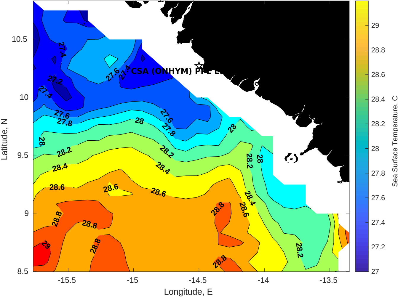
SST for CSA (ONHYM) PPL EBS - Guinea at 09-Dec-2025 00:00:00
