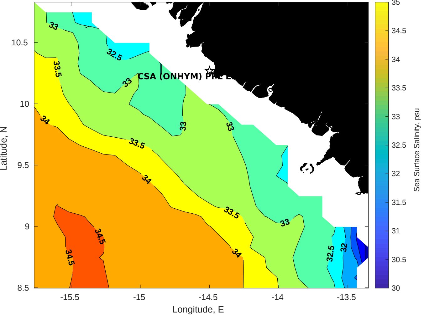
Surface Salinity for CSA (ONHYM) PPL EBS - Guinea at 09-Dec-2025 00:00:00
