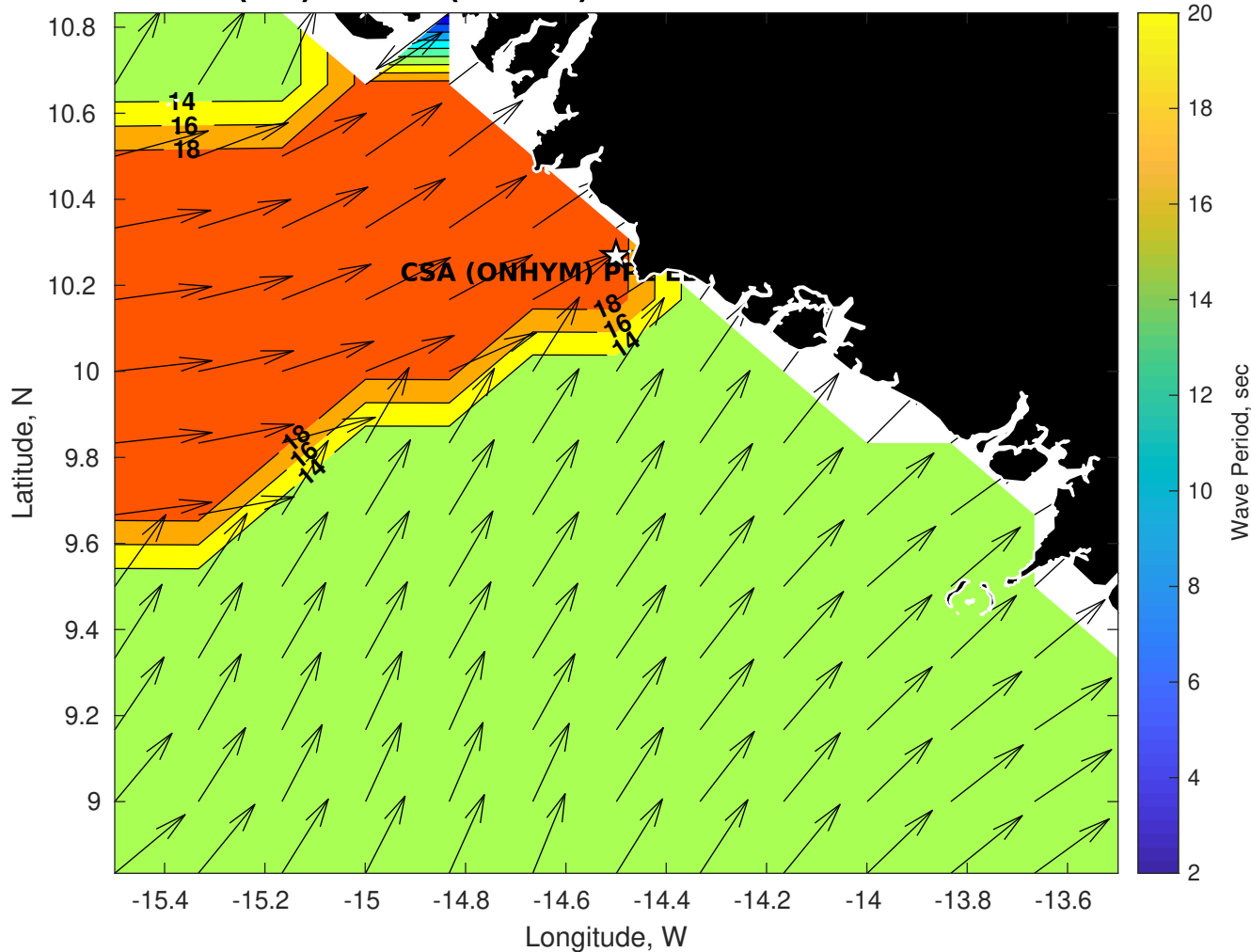
GFS Wave Period (sec) for CSA (ONHYM) PPL EBS - Guinea at 10-Dec-2025 09:00:00
