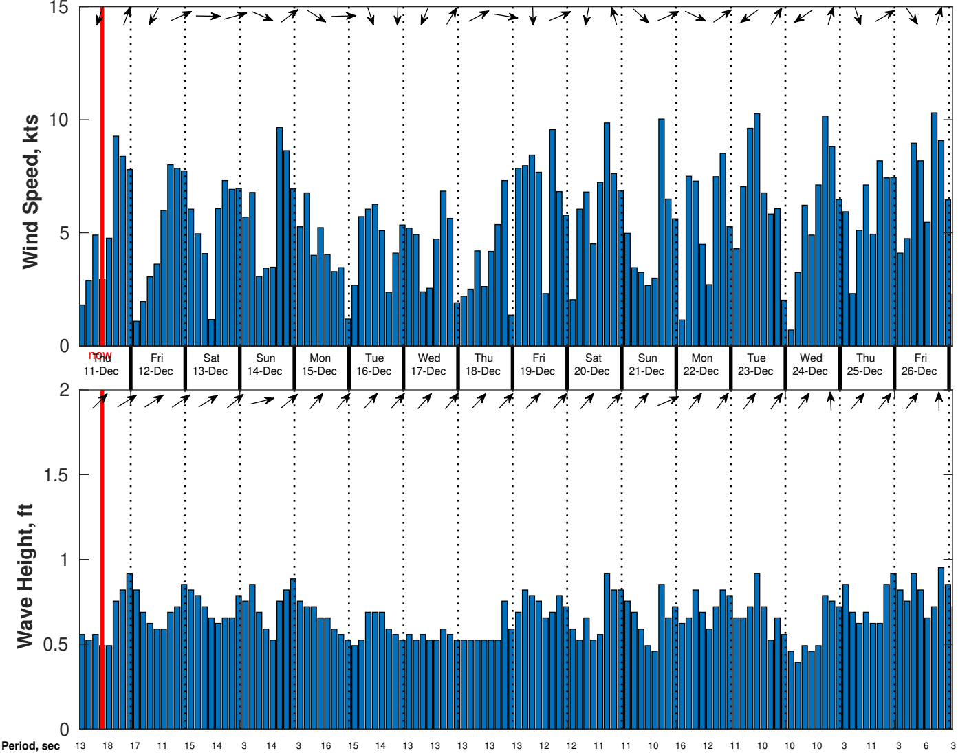
Wind & Wave Forecast for CSA (ONHYM) PPL EBS - Guinea from 10-Dec-2025 01:00:00 to 26-Dec-2025 01:00:00
