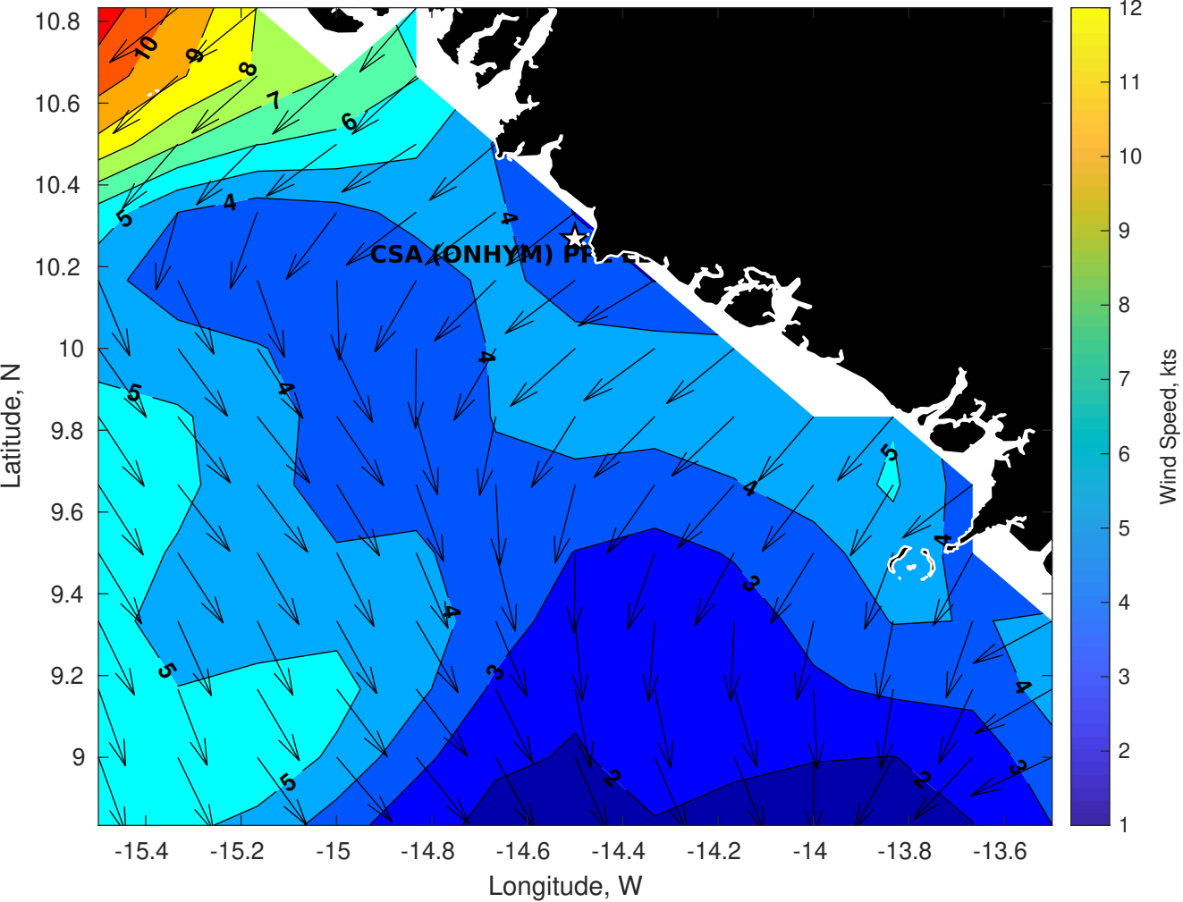
GFS Winds (kts) for CSA (ONHYM) PPL EBS - Guinea at 10-Dec-2025 09:00:00
