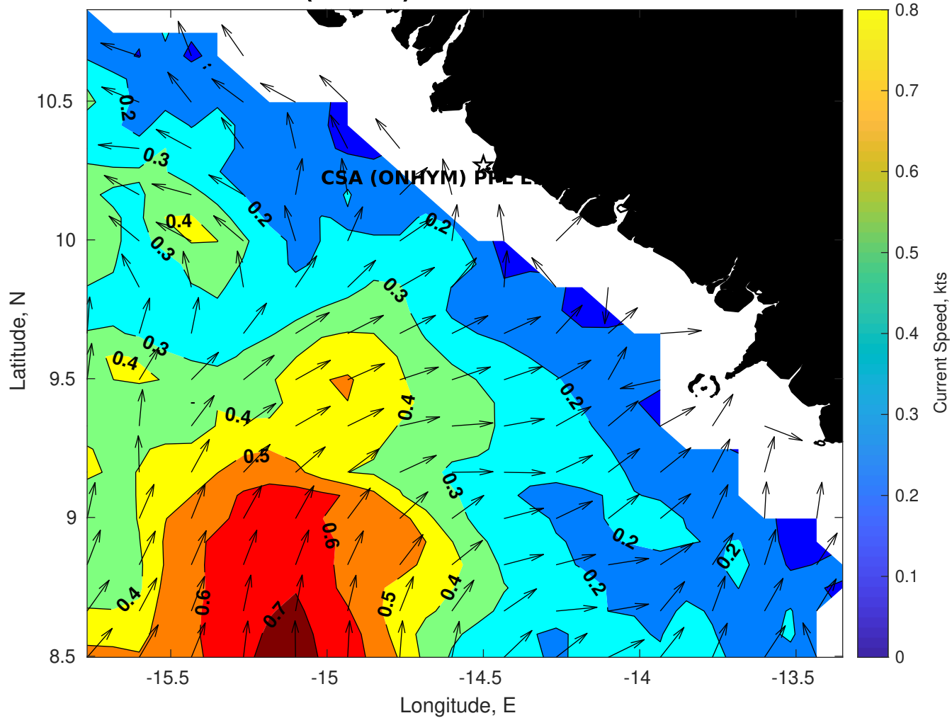
Surface Currents for CSA (ONHYM) PPL EBS - Guinea at 09-Dec-2025 00:00:00
