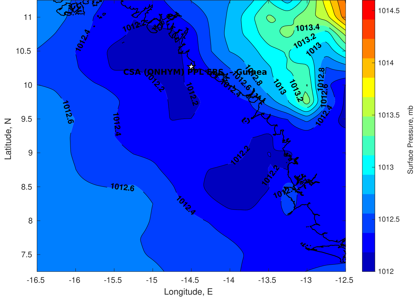
Surface Pressure (mb) for CSA (ONHYM) PPL EBS - Guinea at 12-Dec-2025 00:00:00
