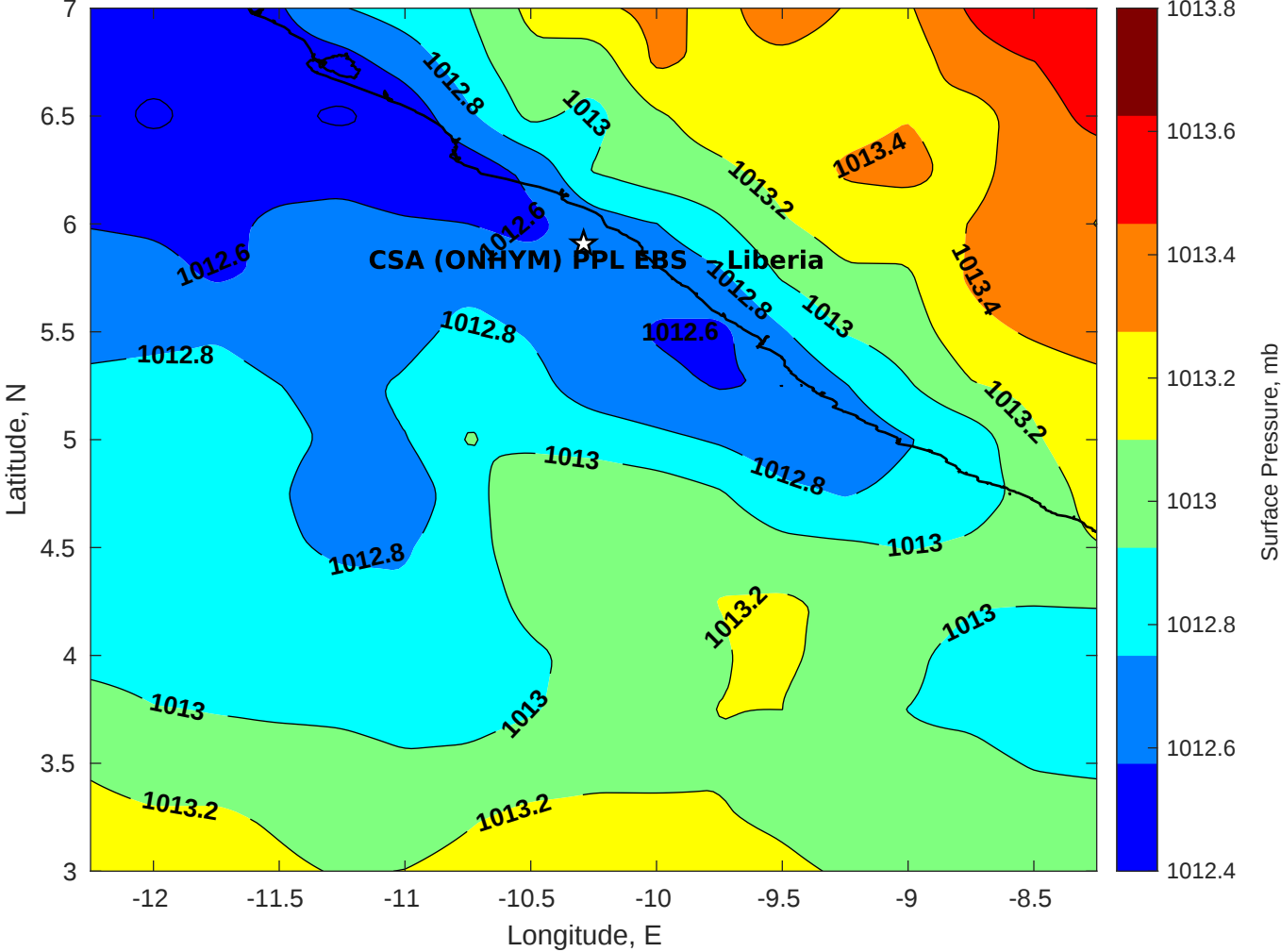
Surface Pressure (mb) for CSA (ONHYM) PPL EBS - Liberia at 10-Dec-2025 00:00:00
