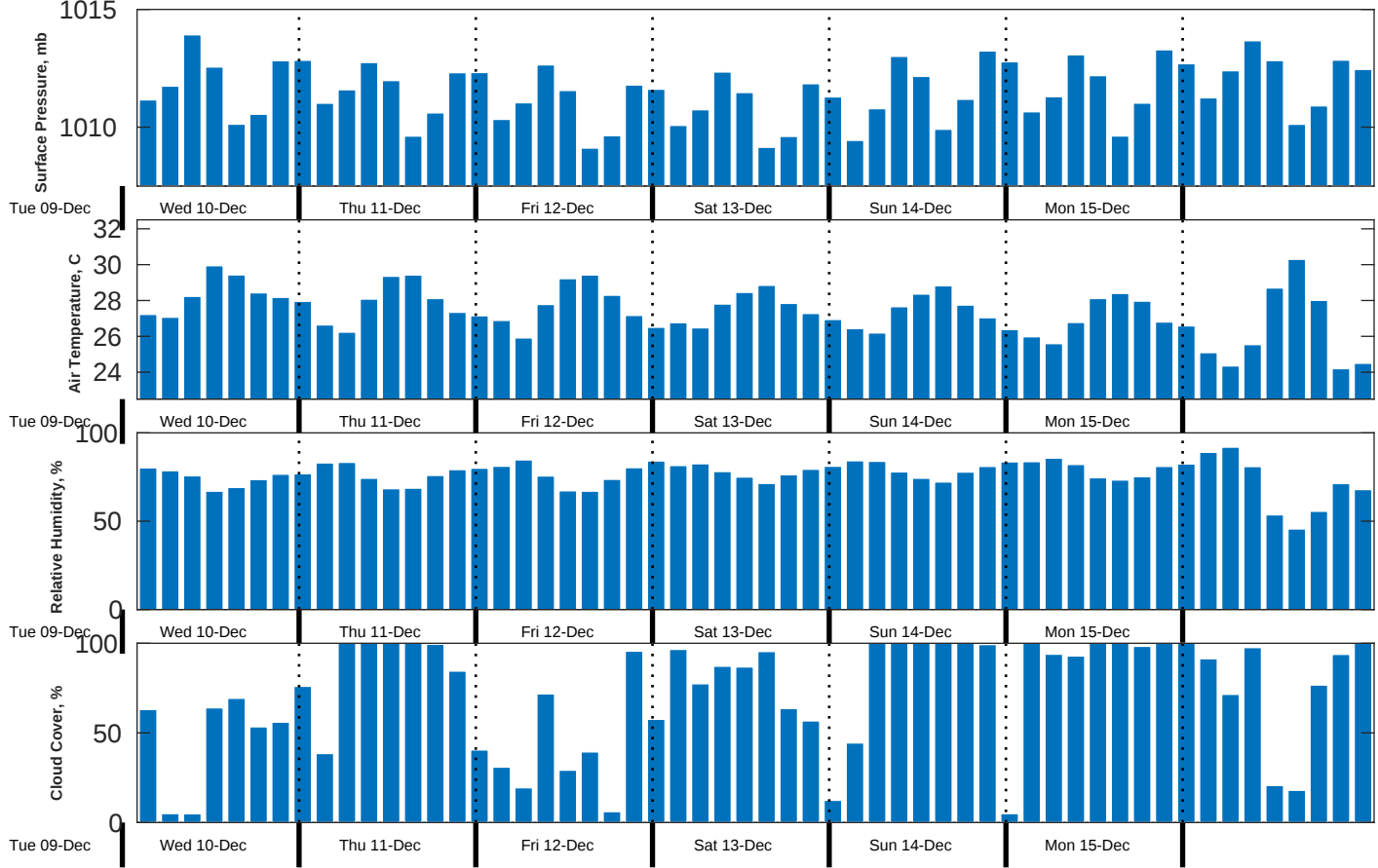
Met Forecast for CSA (ONHYM) PPL EBS - Liberia from 10-Dec-2025 00:00:00 to 17-Dec-2025 00:00:00
