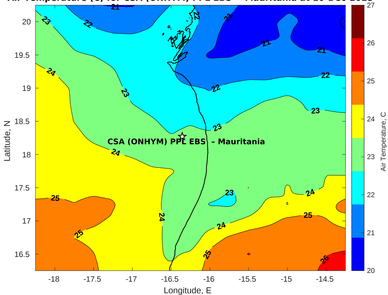
Air Temperature (C) for CSA (ONHYM) PPL EBS - Mauritania at 10-Dec-2025
