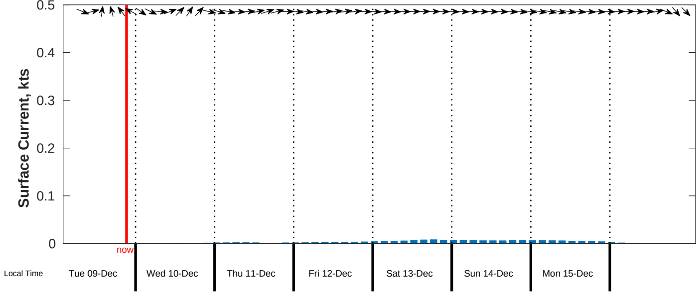
Surface Current Forecast for CSA (ONHYM) PPL EBS - Mauritania from 09-Dec-2025 00:00:00 to 17-Dec-2025 00:00:00
