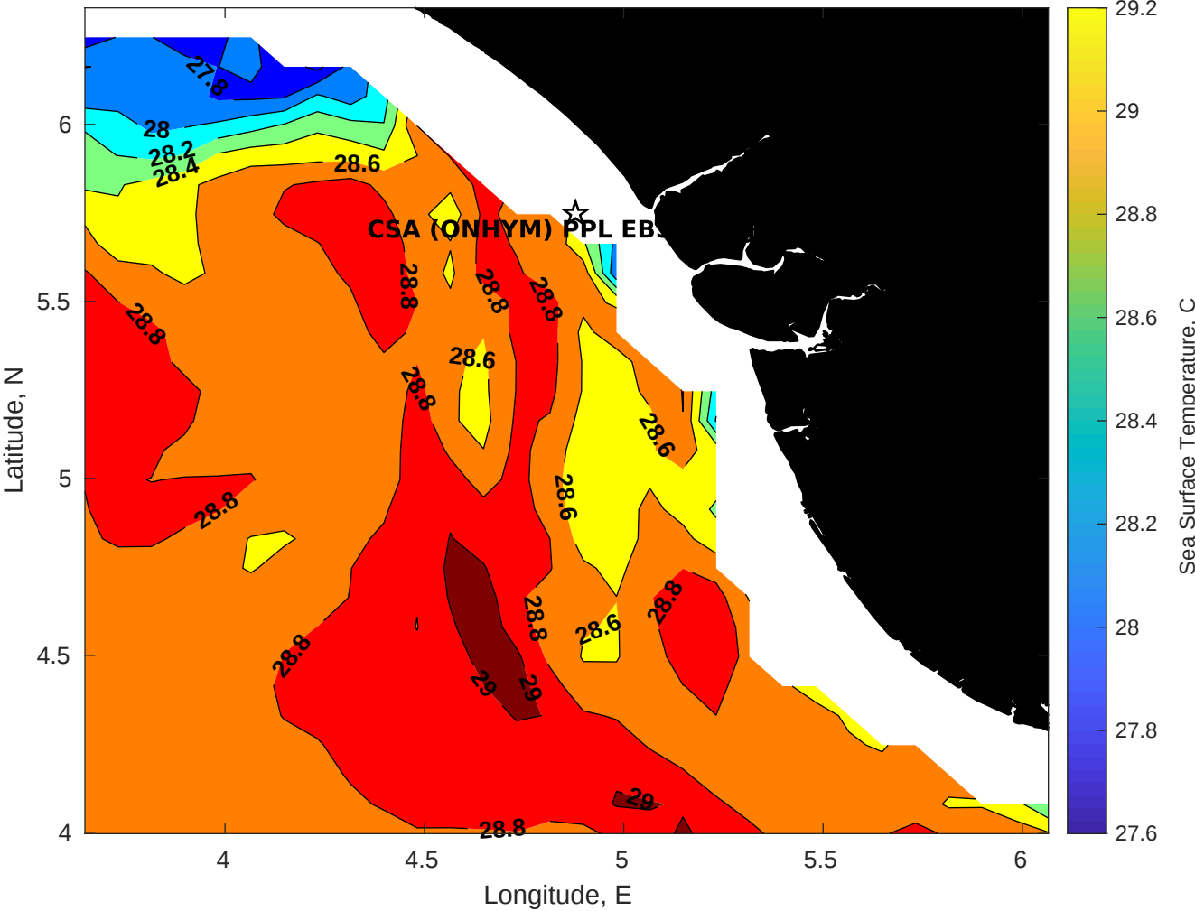
SST for CSA (ONHYM) PPL EBS - Nigeria at 09-Dec-2025 00:00:00
