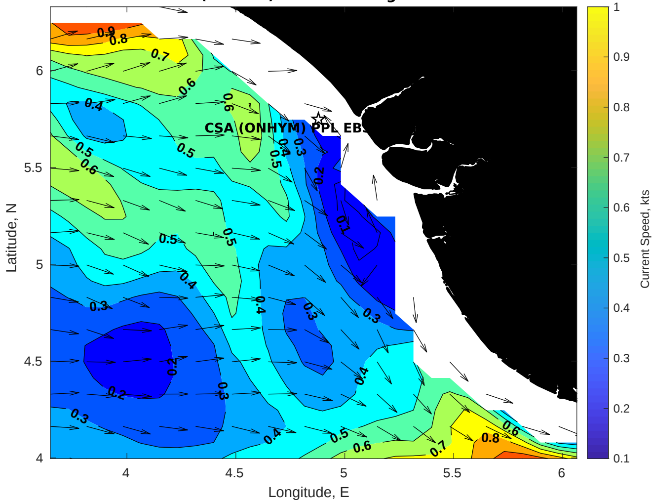
Surface Currents for CSA (ONHYM) PPL EBS - Nigeria at 09-Dec-2025 00:00:00
