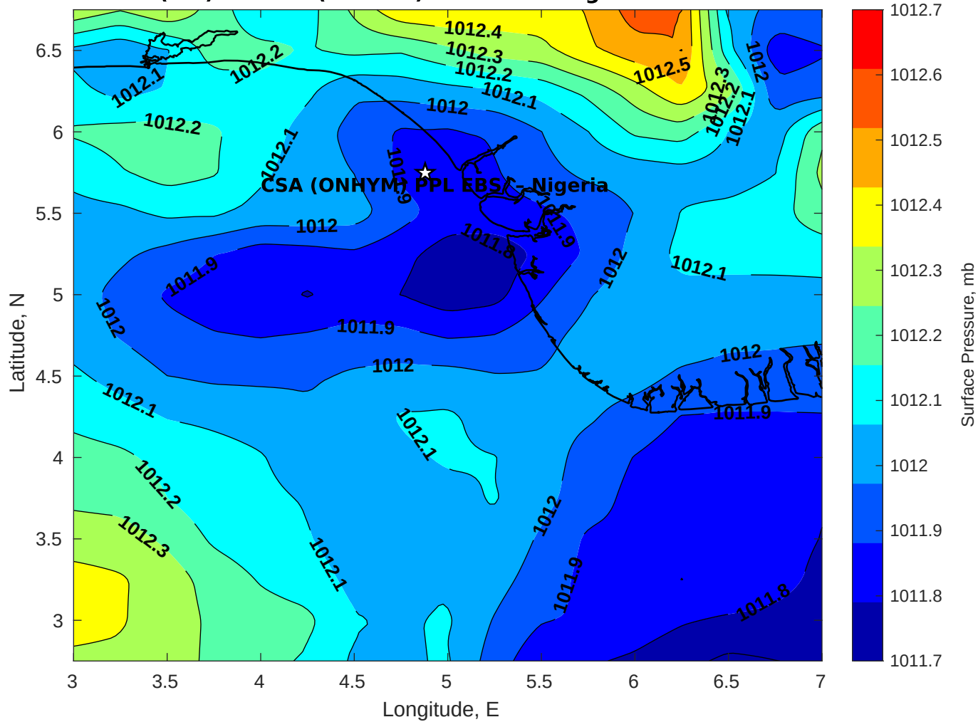
Surface Pressure (mb) for CSA (ONHYM) PPL EBS - Nigeria at 10-Dec-2025 00:00:00
