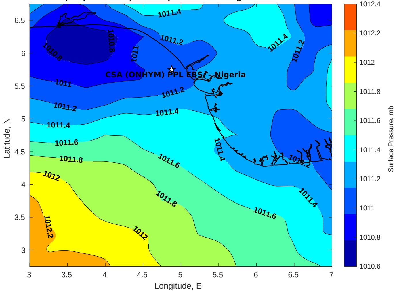
Surface Pressure (mb) for CSA (ONHYM) PPL EBS - Nigeria at 11-Dec-2025 00:00:00
