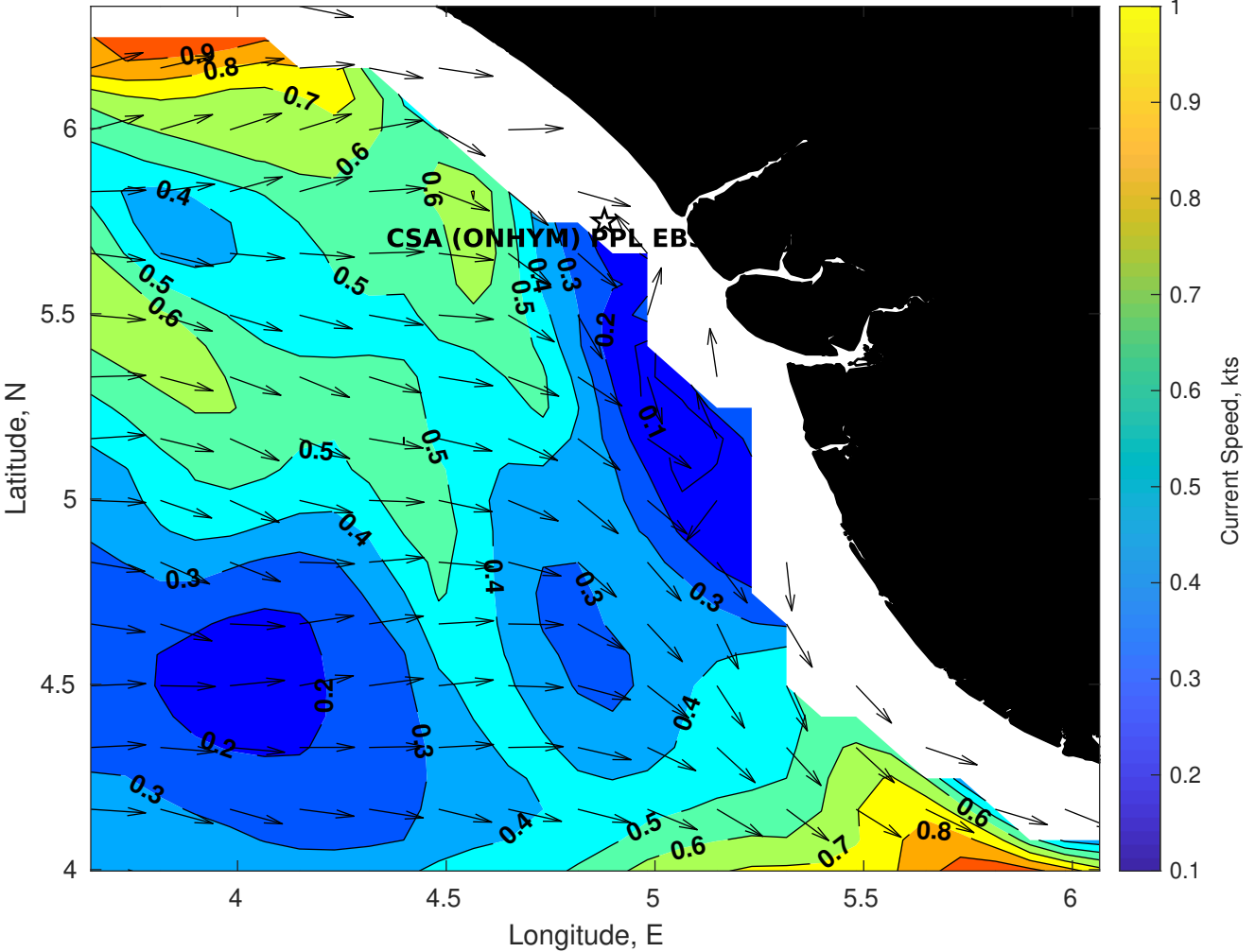
Surface Currents for CSA (ONHYM) PPL EBS - Nigeria at 09-Dec-2025 00:00:00
