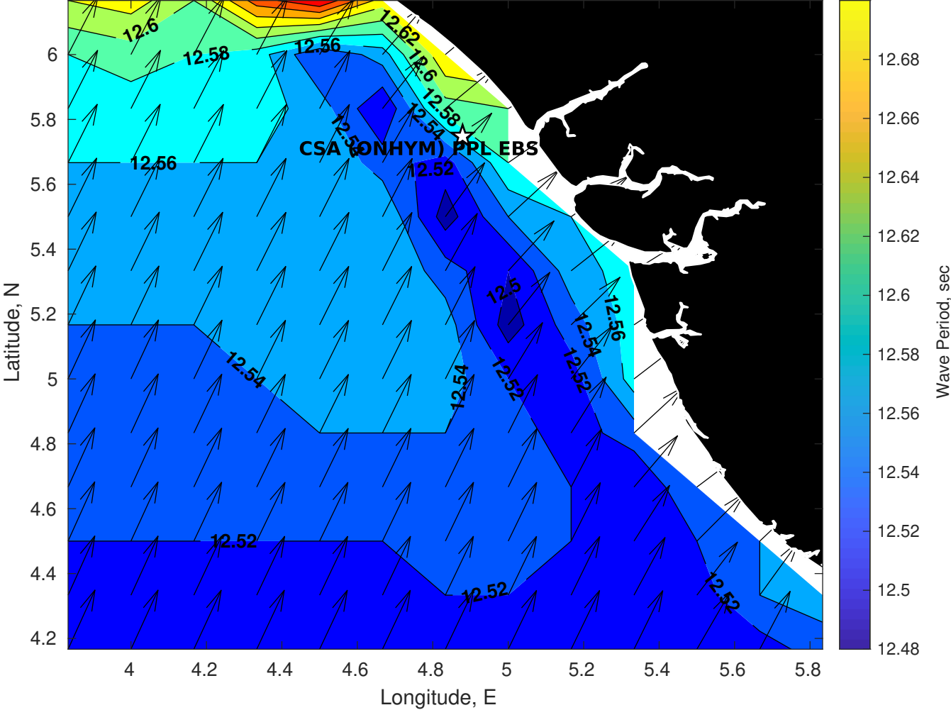
GFS Wave Period (sec) for CSA (ONHYM) PPL EBS - Nigeria at 10-Dec-2025 09:00:00
