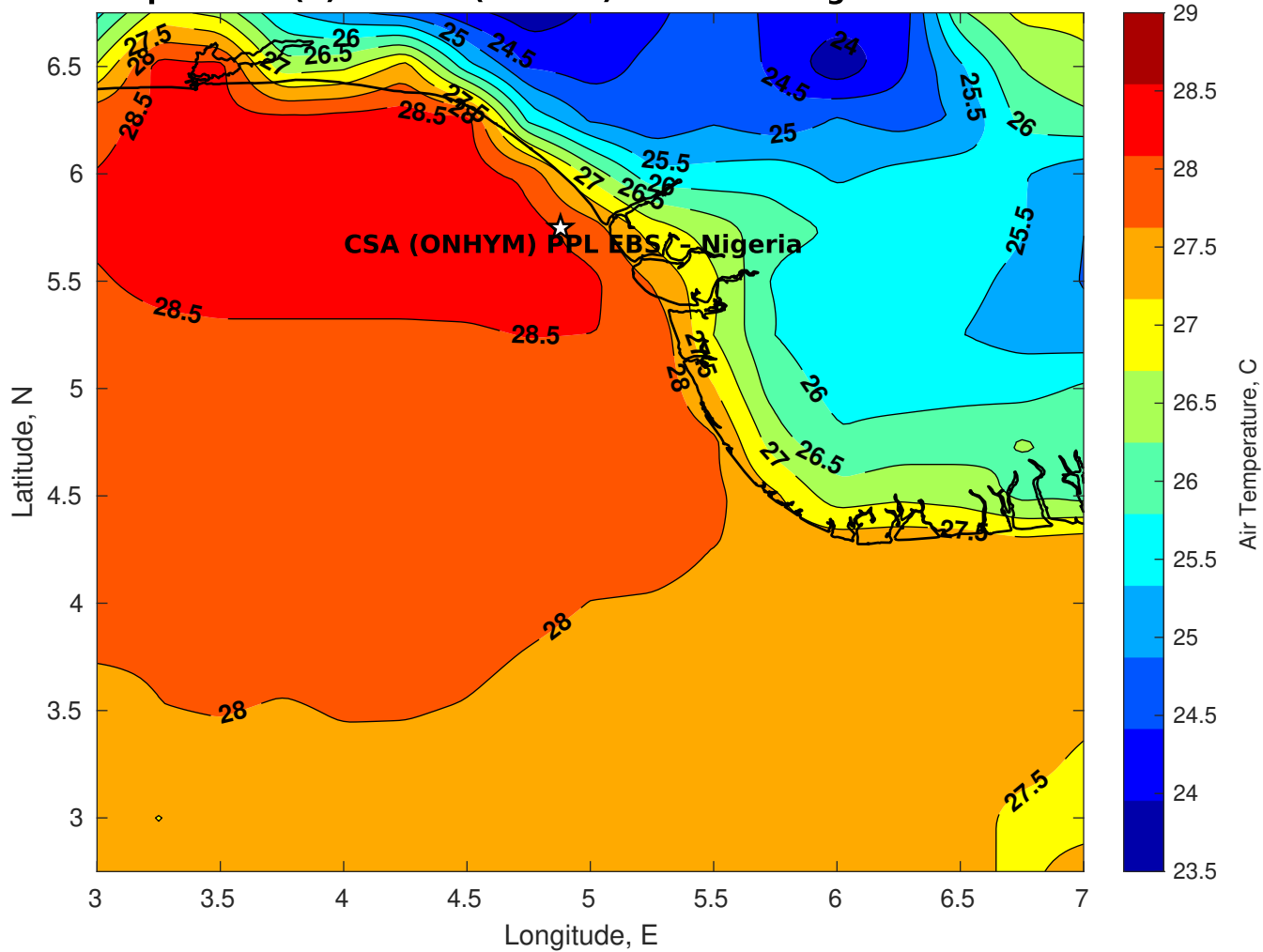
Air Temperature (C) for CSA (ONHYM) PPL EBS - Nigeria at 10-Dec-2025
