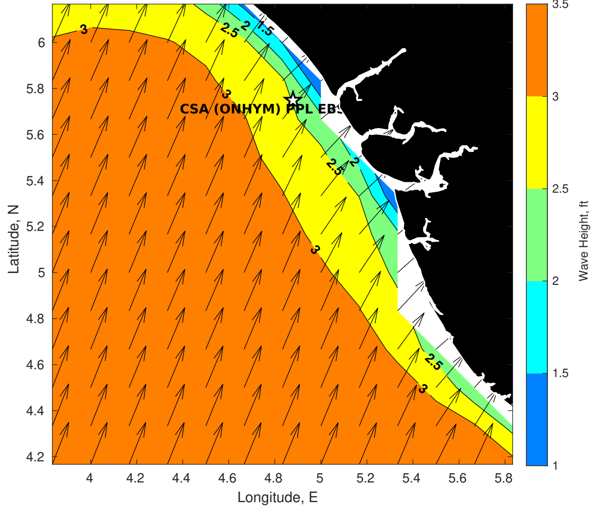
GFS Wave Height (ft) for CSA (ONHYM) PPL EBS - Nigeria at 10-Dec-2025 09:00:00
