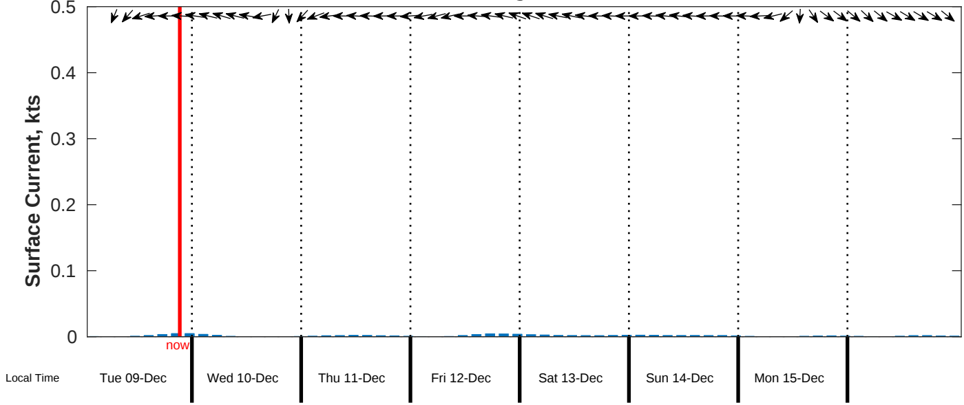
Surface Current Forecast for CSA (ONHYM) PPL EBS - Nigeria from 09-Dec-2025 00:00:00 to 17-Dec-2025 00:00:00
