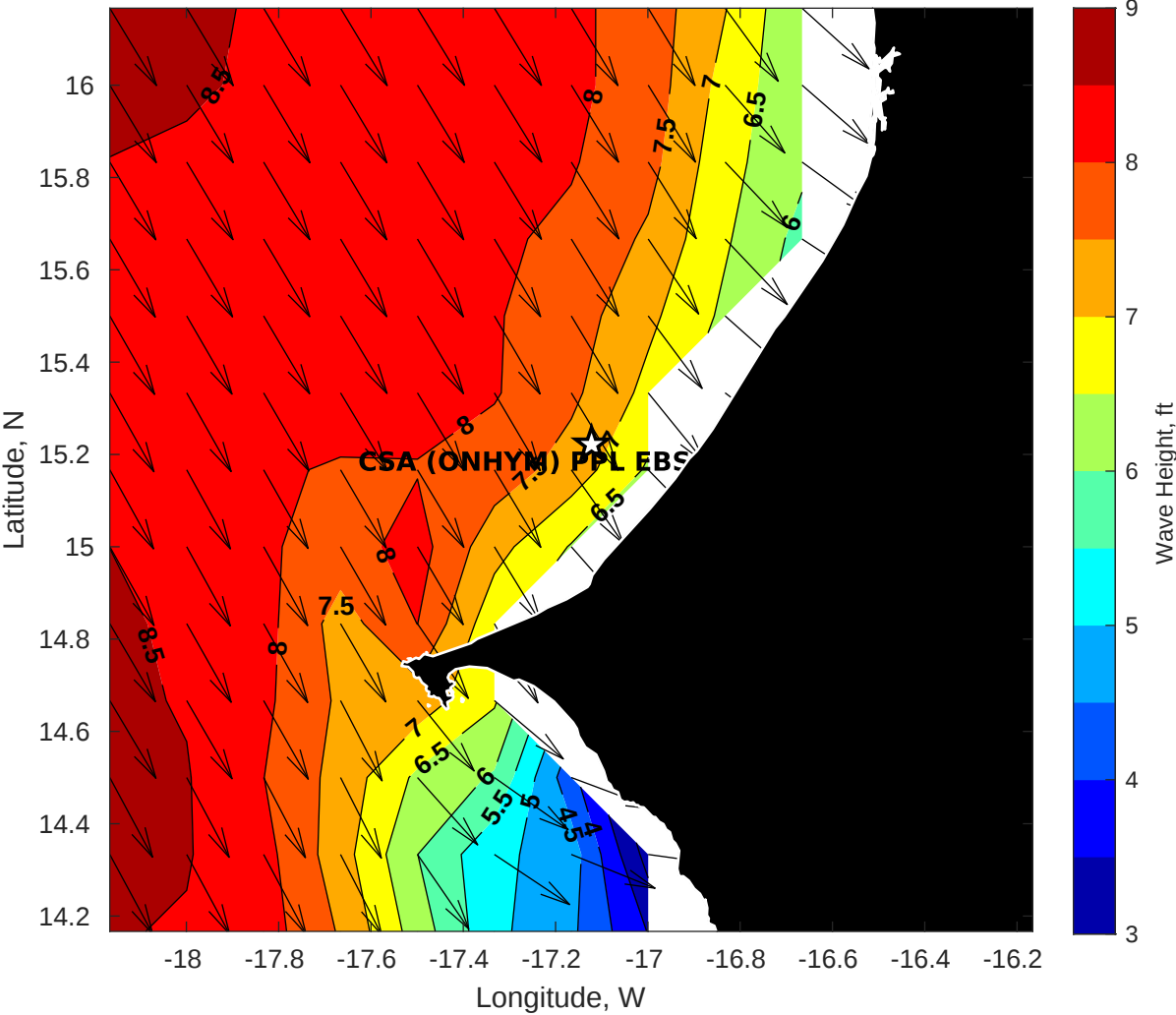
GFS Wave Height (ft) for CSA (ONHYM) PPL EBS - Senegal at 10-Dec-2025 09:00:00
