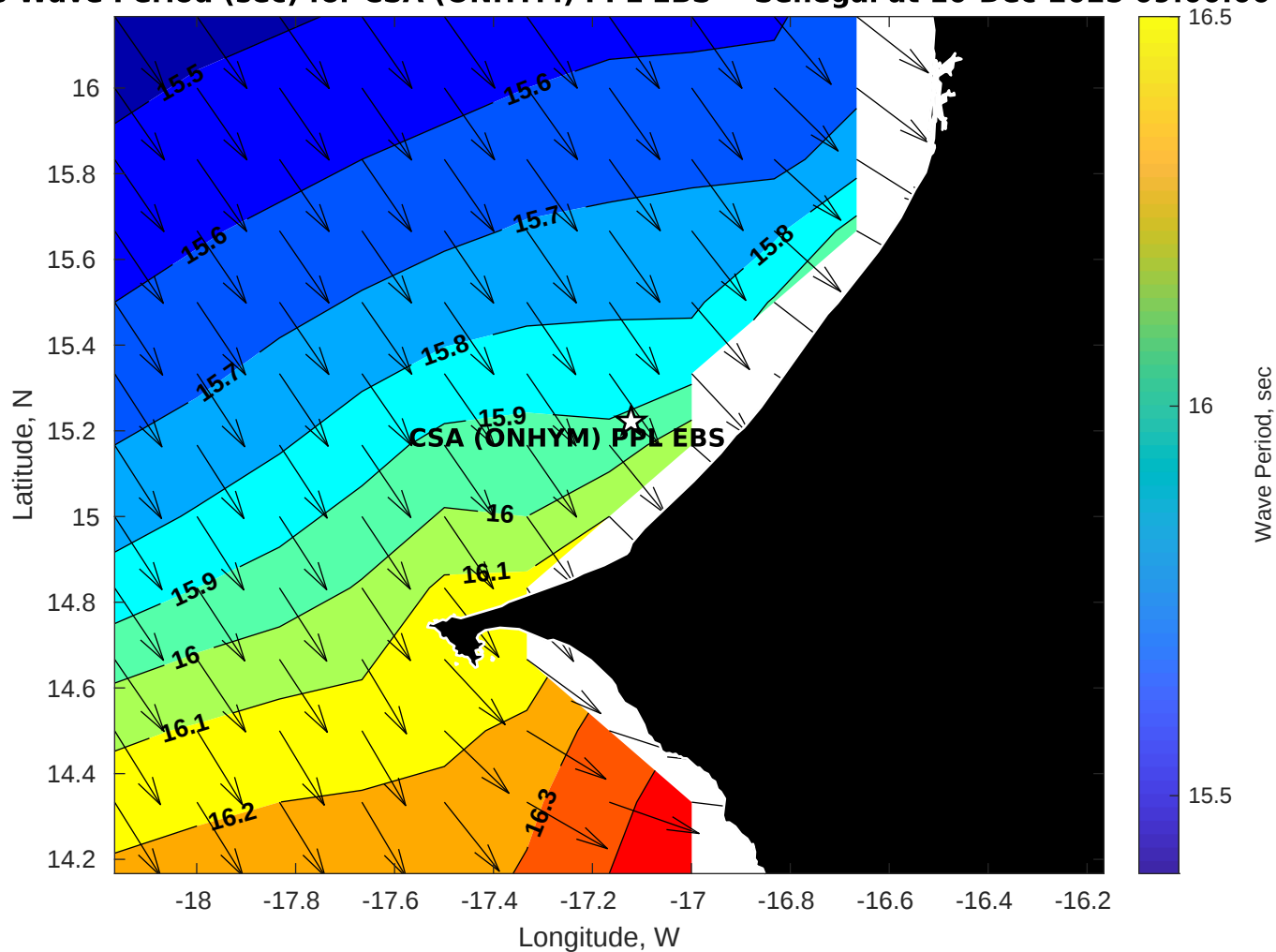
GFS Wave Period (sec) for CSA (ONHYM) PPL EBS - Senegal at 10-Dec-2025 09:00:00
