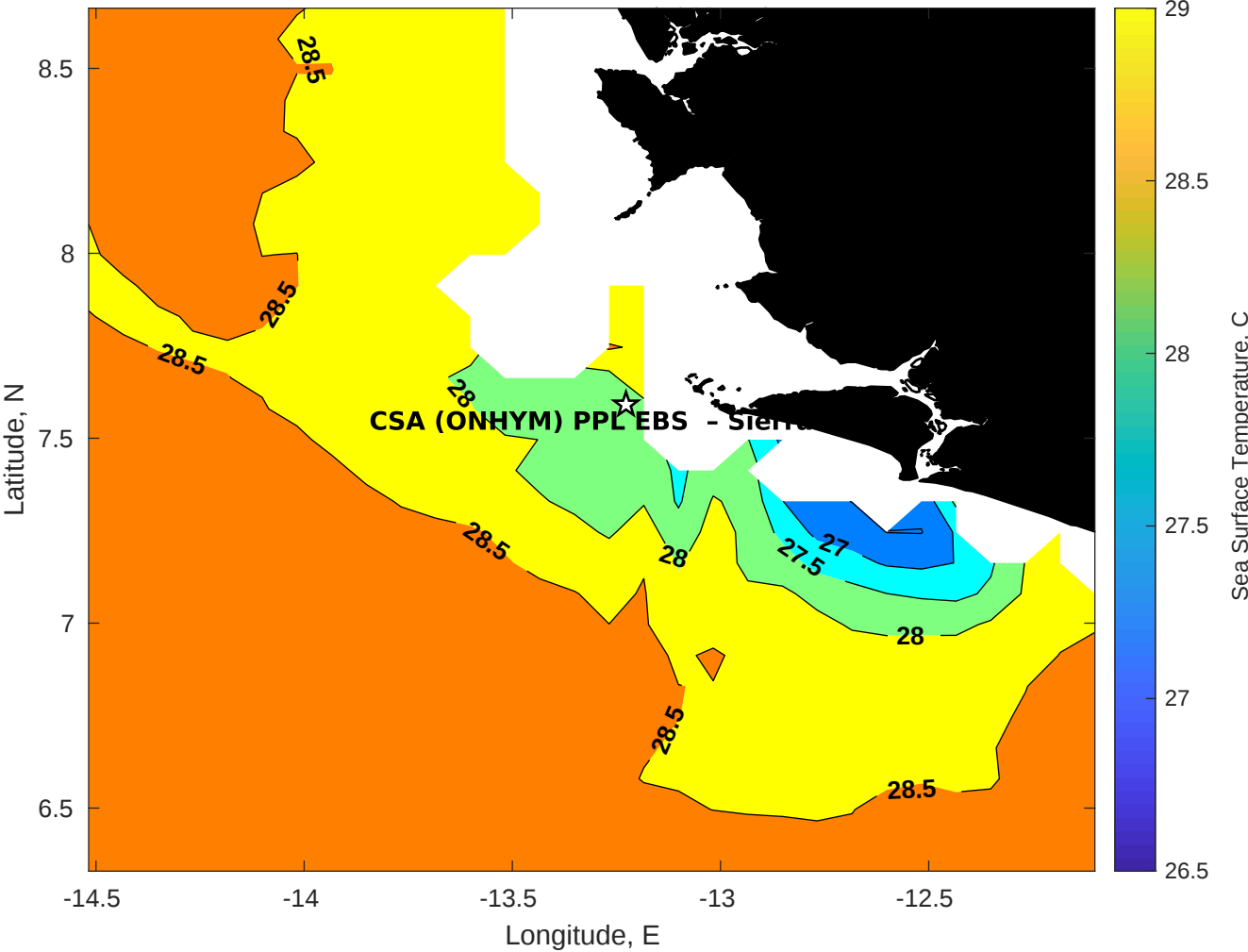
SST for CSA (ONHYM) PPL EBS - Sierra Leone at 09-Dec-2025 00:00:00
