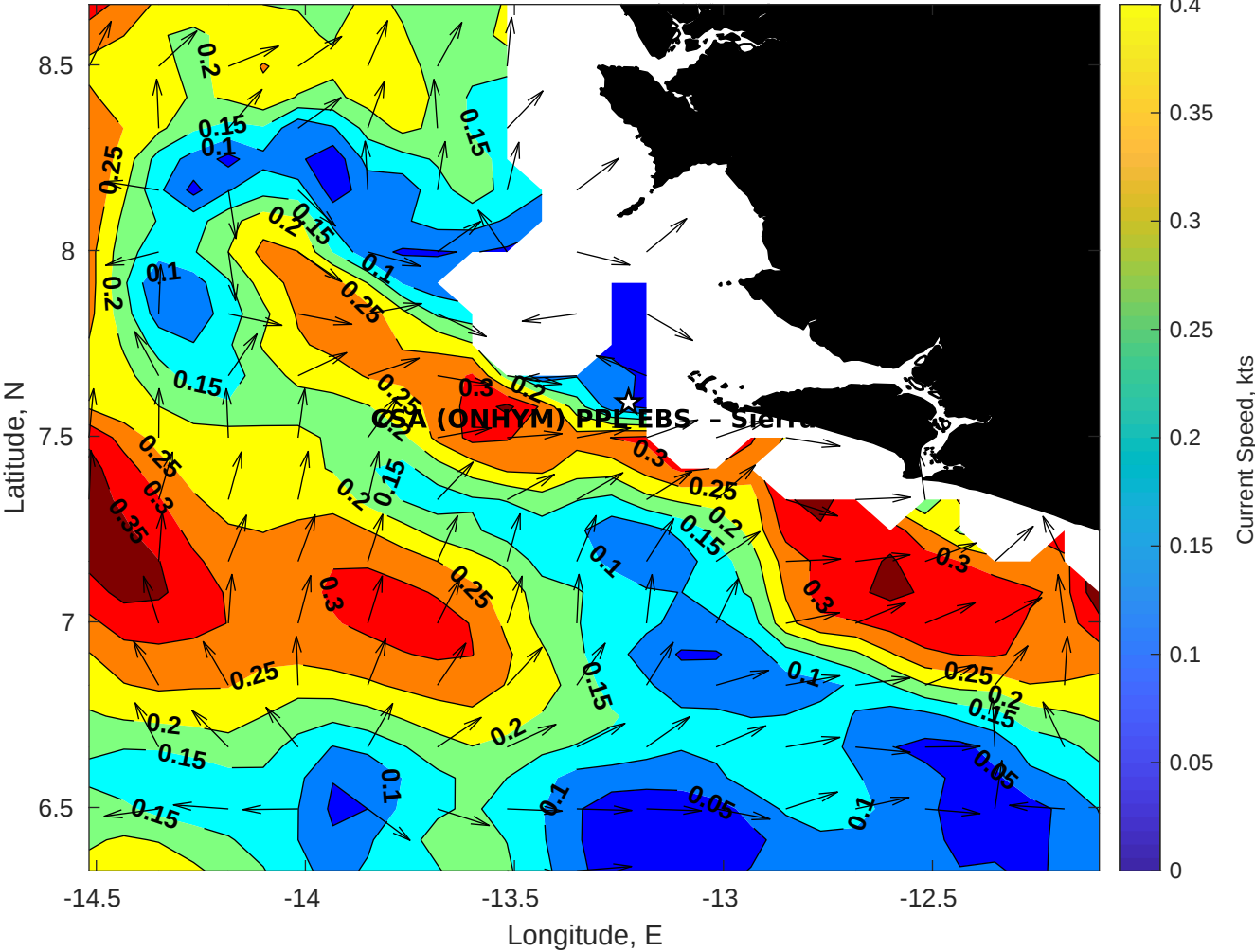
Surface Currents for CSA (ONHYM) PPL EBS - Sierra Leone at 09-Dec-2025 00:00:00
