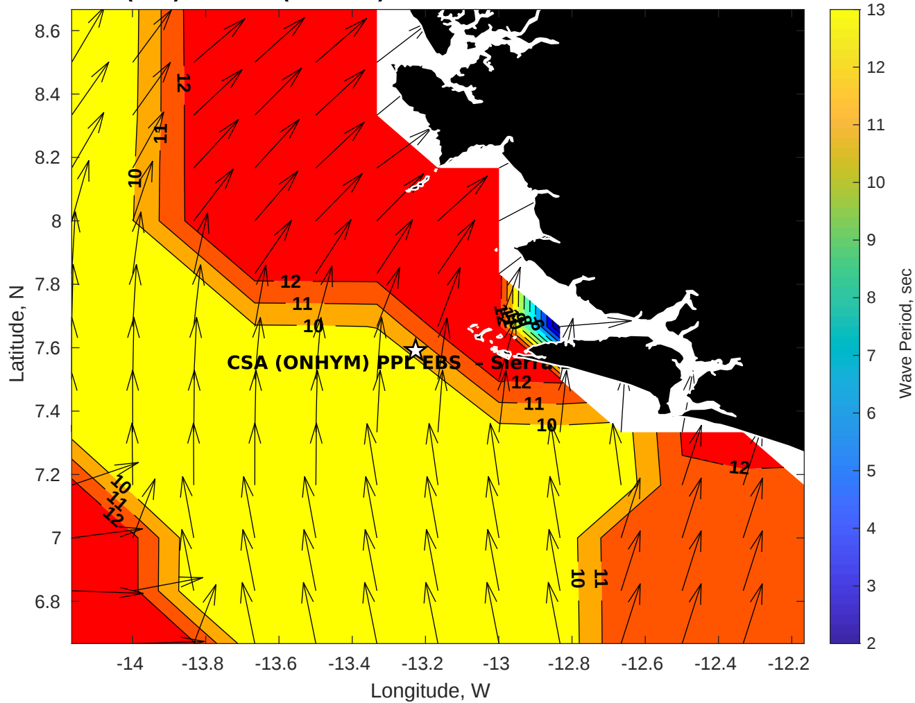
GFS Wave Period (sec) for CSA (ONHYM) PPL EBS - Sierra Leone at 10-Dec-2025 09:00:00
