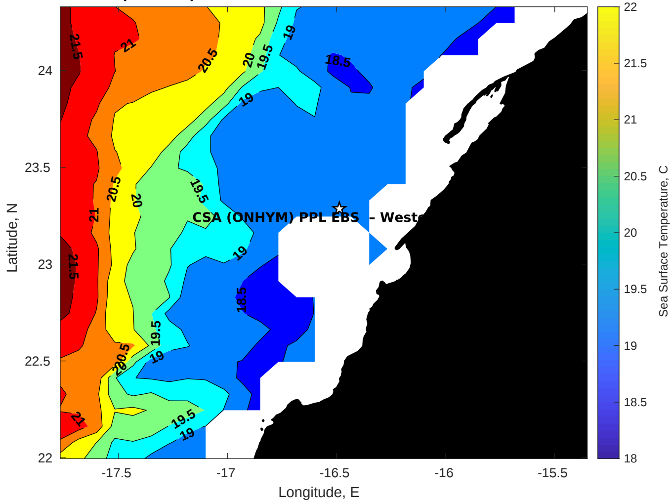
SST for CSA (ONHYM) PPL EBS - Western Sahara at 09-Dec-2025 00:00:00
