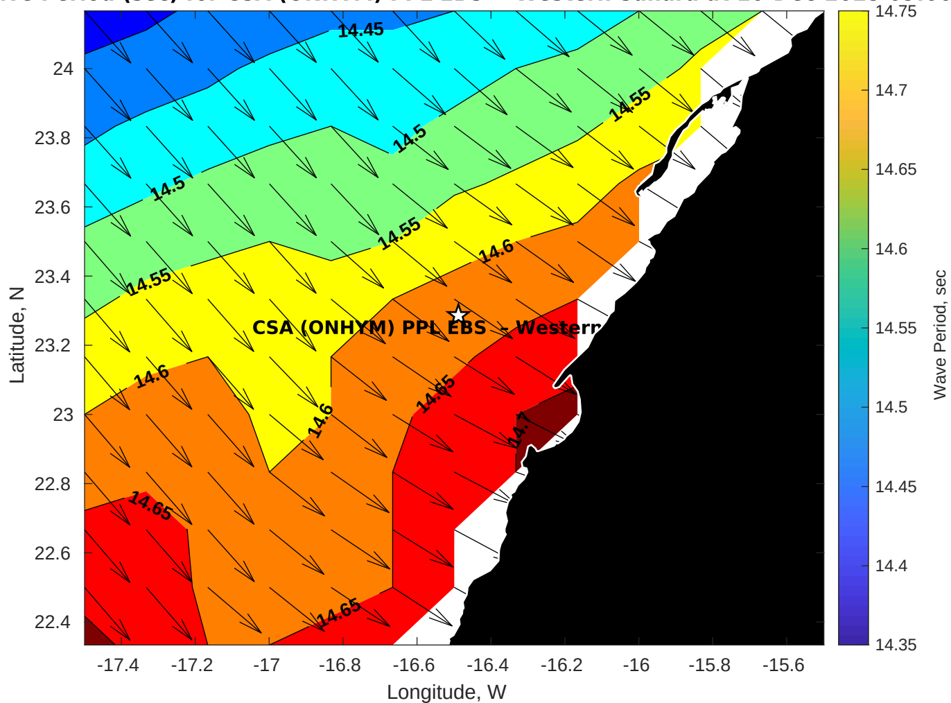
GFS Wave Period (sec) for CSA (ONHYM) PPL EBS - Western Sahara at 10-Dec-2025 09:00:00
