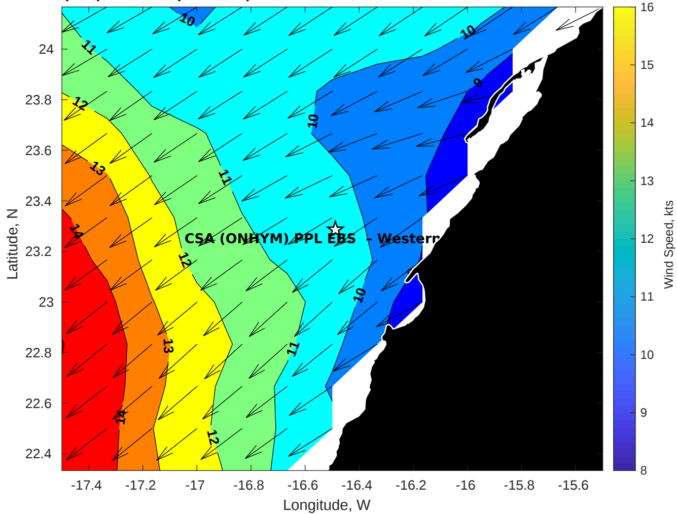
GFS Winds (kts) for CSA (ONHYM) PPL EBS - Western Sahara at 10-Dec-2025 09:00:00
