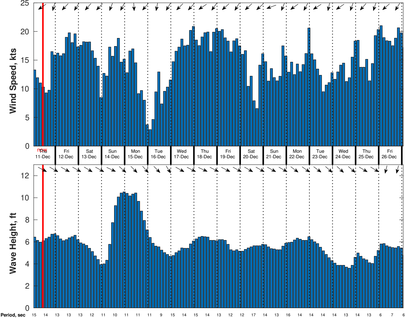
Wind & Wave Forecast for CSA (ONHYM) PPL EBS - Western Sahara from 10-Dec-2025 01:00:00 to 26-Dec-2025 01:00:00
