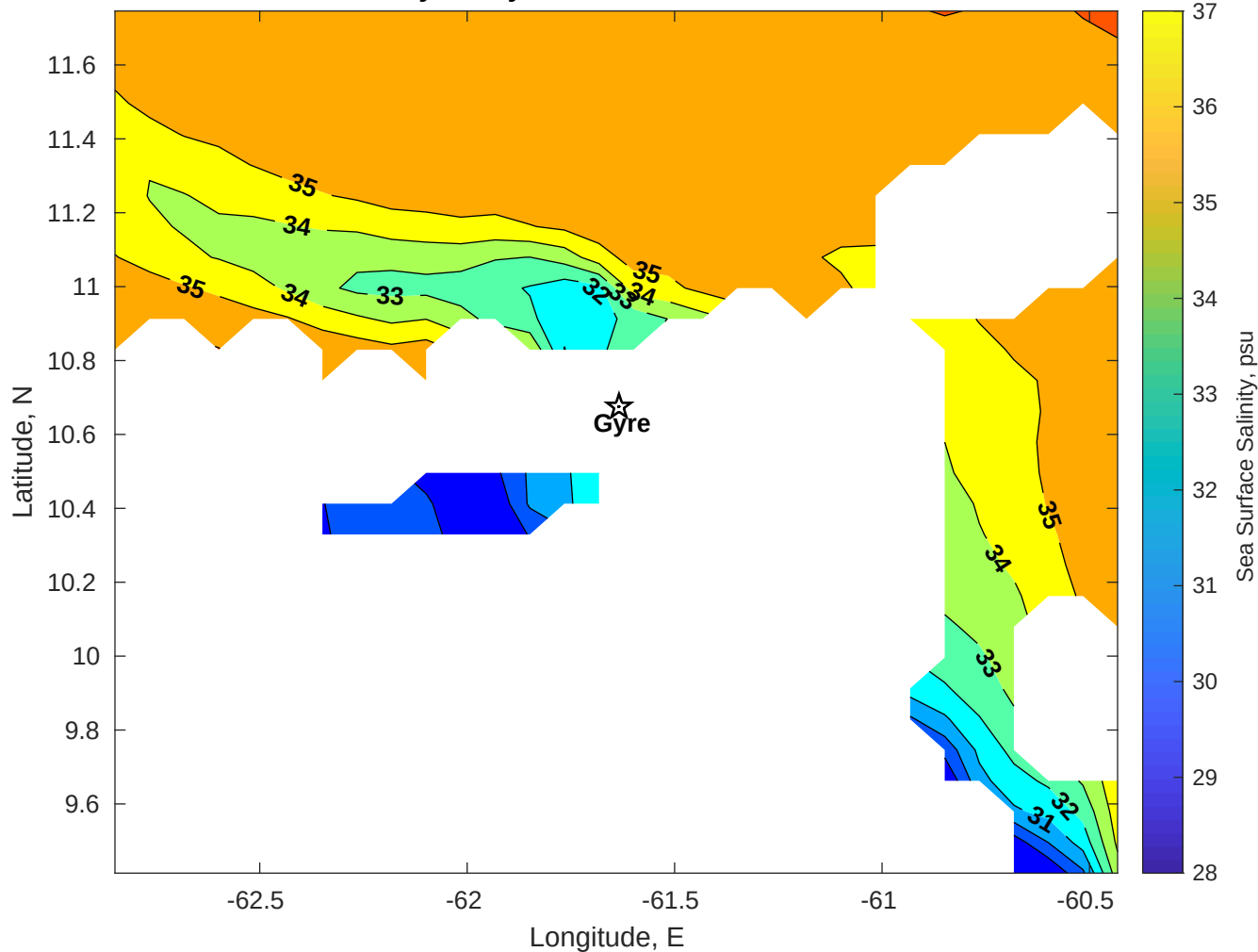
Surface Salinity for Gyre at 09-Dec-2025 00:00:00
