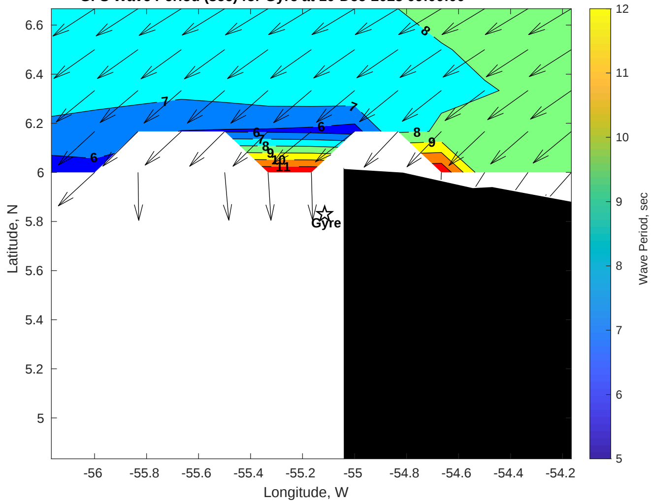
GFS Wave Period (sec) for Gyre at 10-Dec-2025 09:00:00
