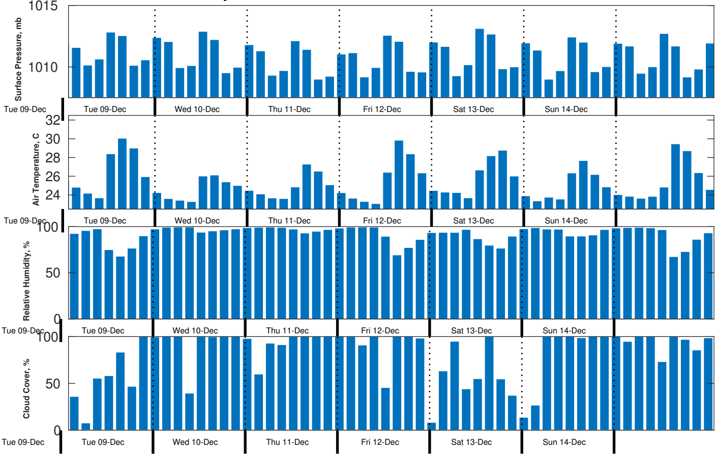
Met Forecast for Gyre from 09-Dec-2025 20:00:00 to 16-Dec-2025 20:00:00
