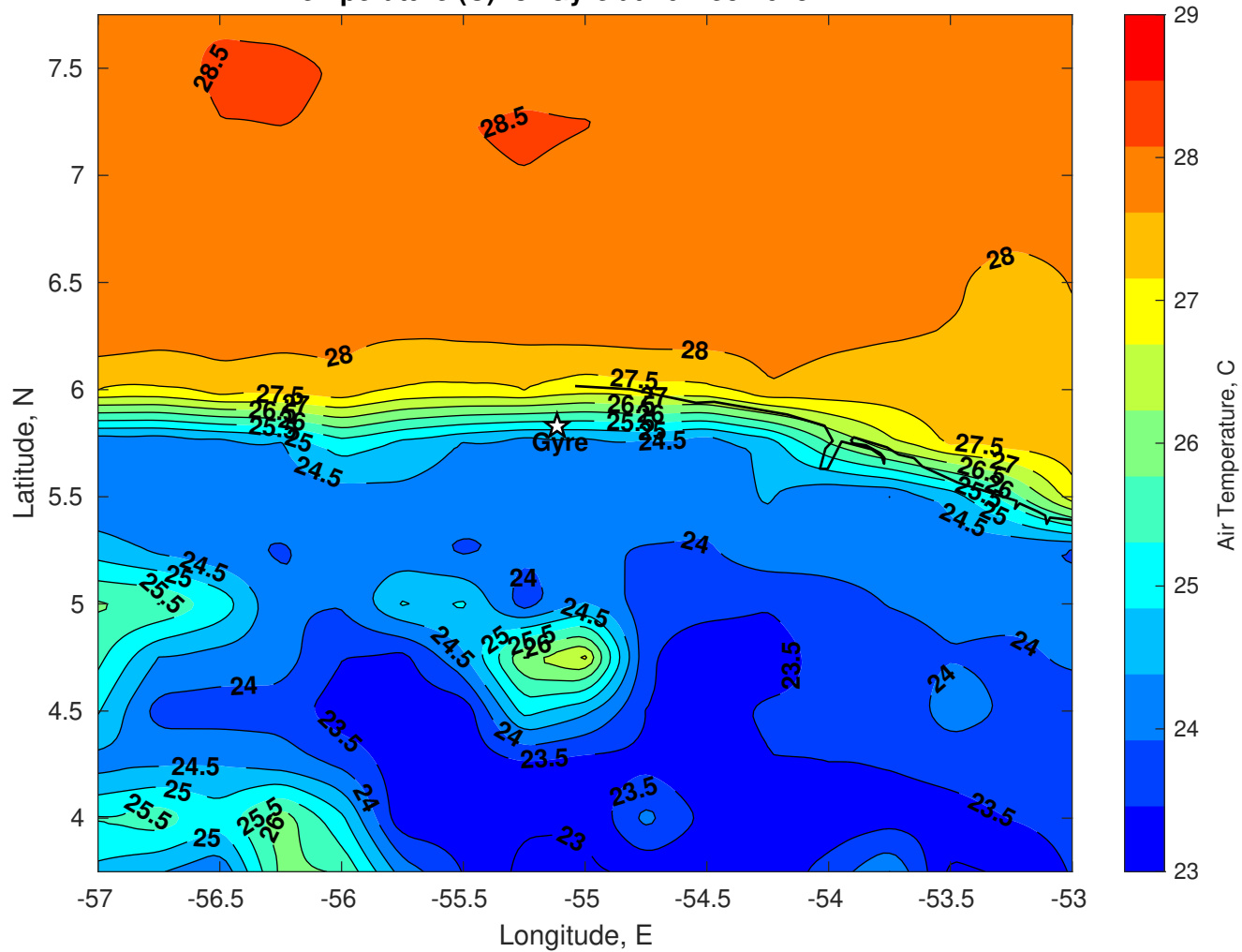
Air Temperature (C) for Gyre at 10-Dec-2025
