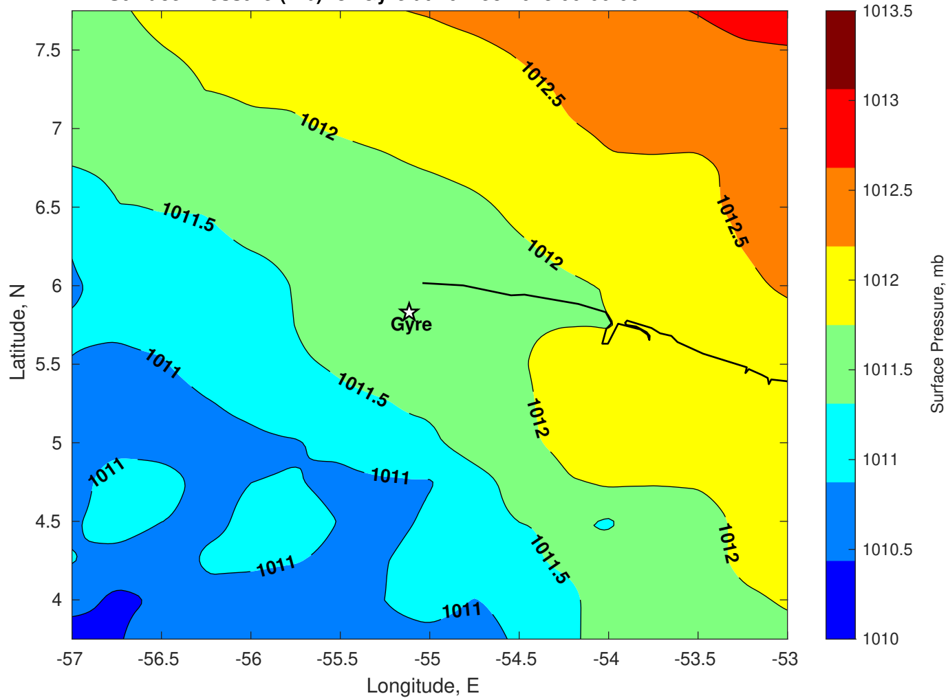
Surface Pressure (mb) for Gyre at 10-Dec-2025 00:00:00
