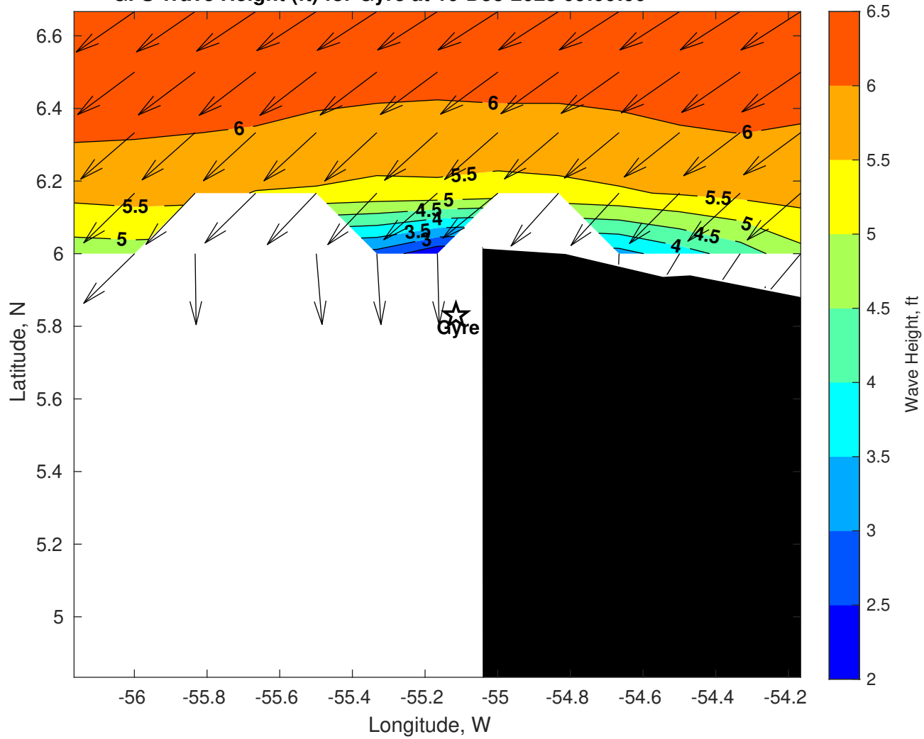
GFS Wave Height (ft) for Gyre at 10-Dec-2025 09:00:00
