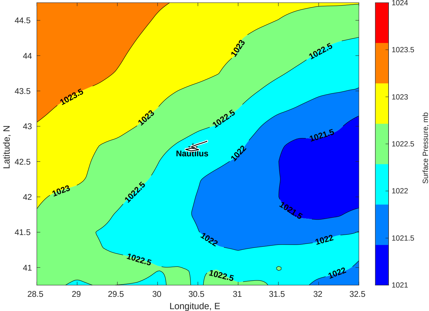
Surface Pressure (mb) for Nautilus at 11-Dec-2025 00:00:00
