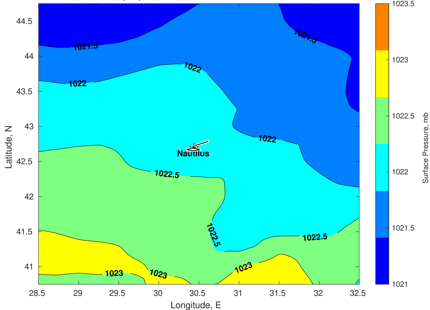
Surface Pressure (mb) for Nautilus at 10-Dec-2025 00:00:00
