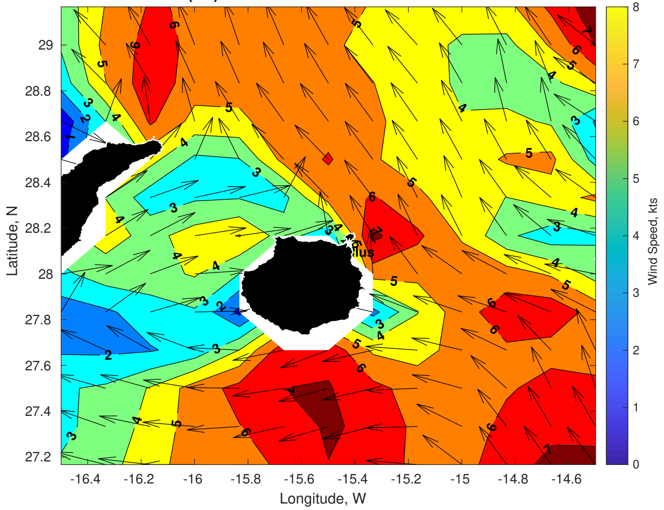
GFS Winds (kts) for Nautilus at 08-Dec-2025 09:00:00
