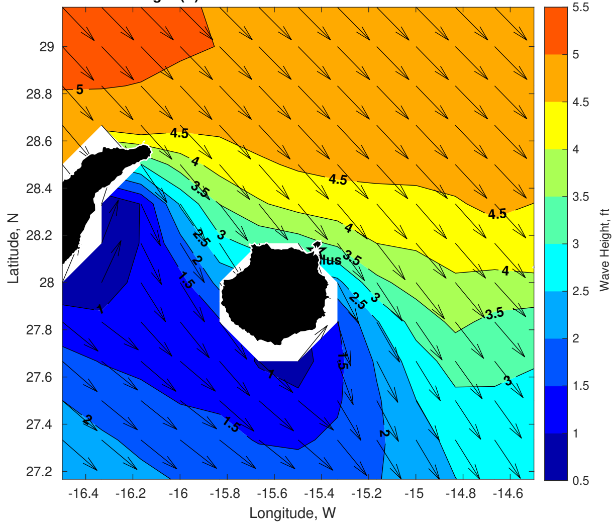
GFS Wave Height (ft) for Nautilus at 08-Dec-2025 09:00:00
