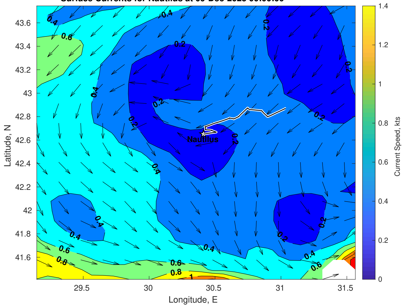
Surface Currents for Nautilus at 09-Dec-2025 00:00:00
