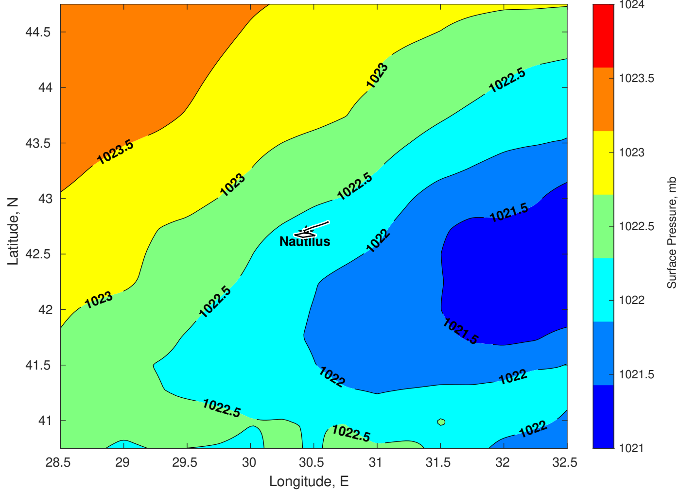
Surface Pressure (mb) for Nautilus at 11-Dec-2025 00:00:00
