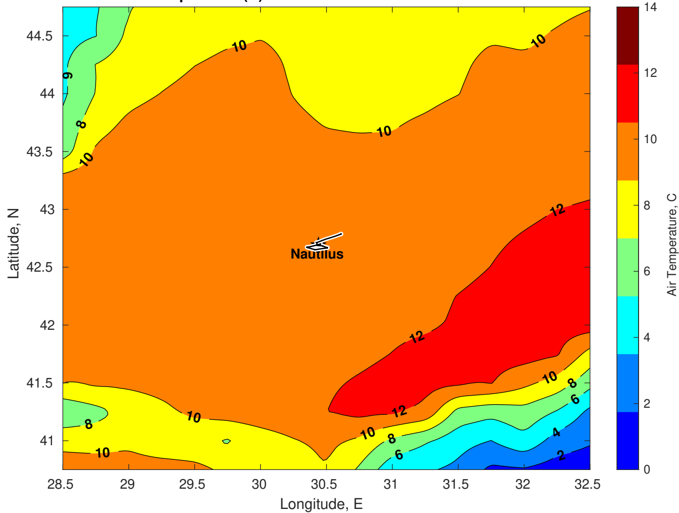
Air Temperature (C) for Nautilus at 10-Dec-2025
