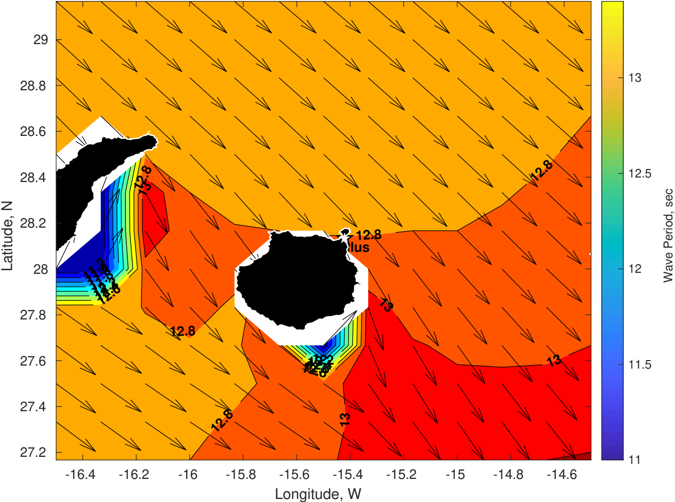
GFS Wave Period (sec) for Nautilus at 08-Dec-2025 09:00:00
