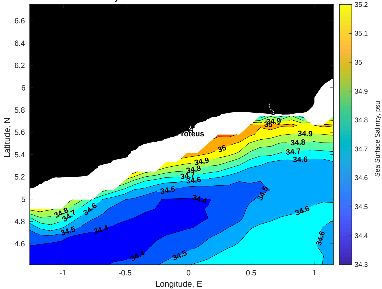
Surface Salinity for Proteus at 09-Dec-2025 00:00:00
