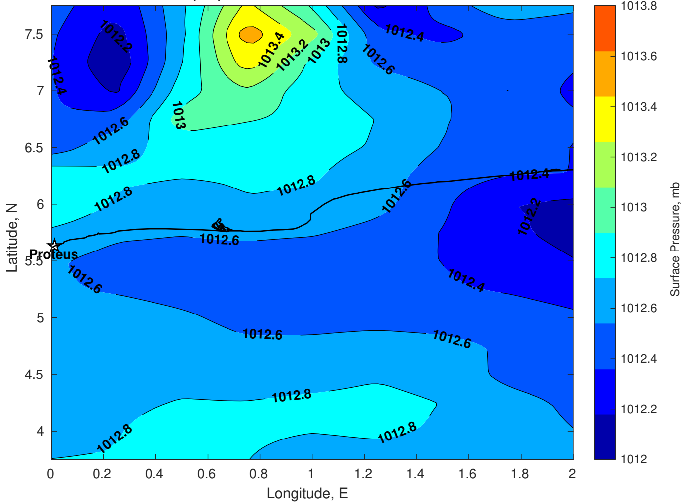
Surface Pressure (mb) for Proteus at 10-Dec-2025 00:00:00
