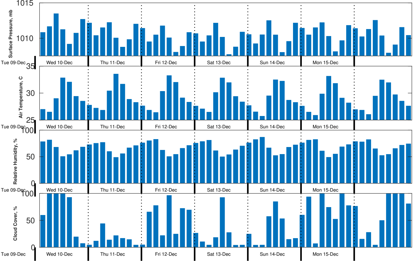
Met Forecast for Proteus from 10-Dec-2025 00:00:00 to 17-Dec-2025 00:00:00
