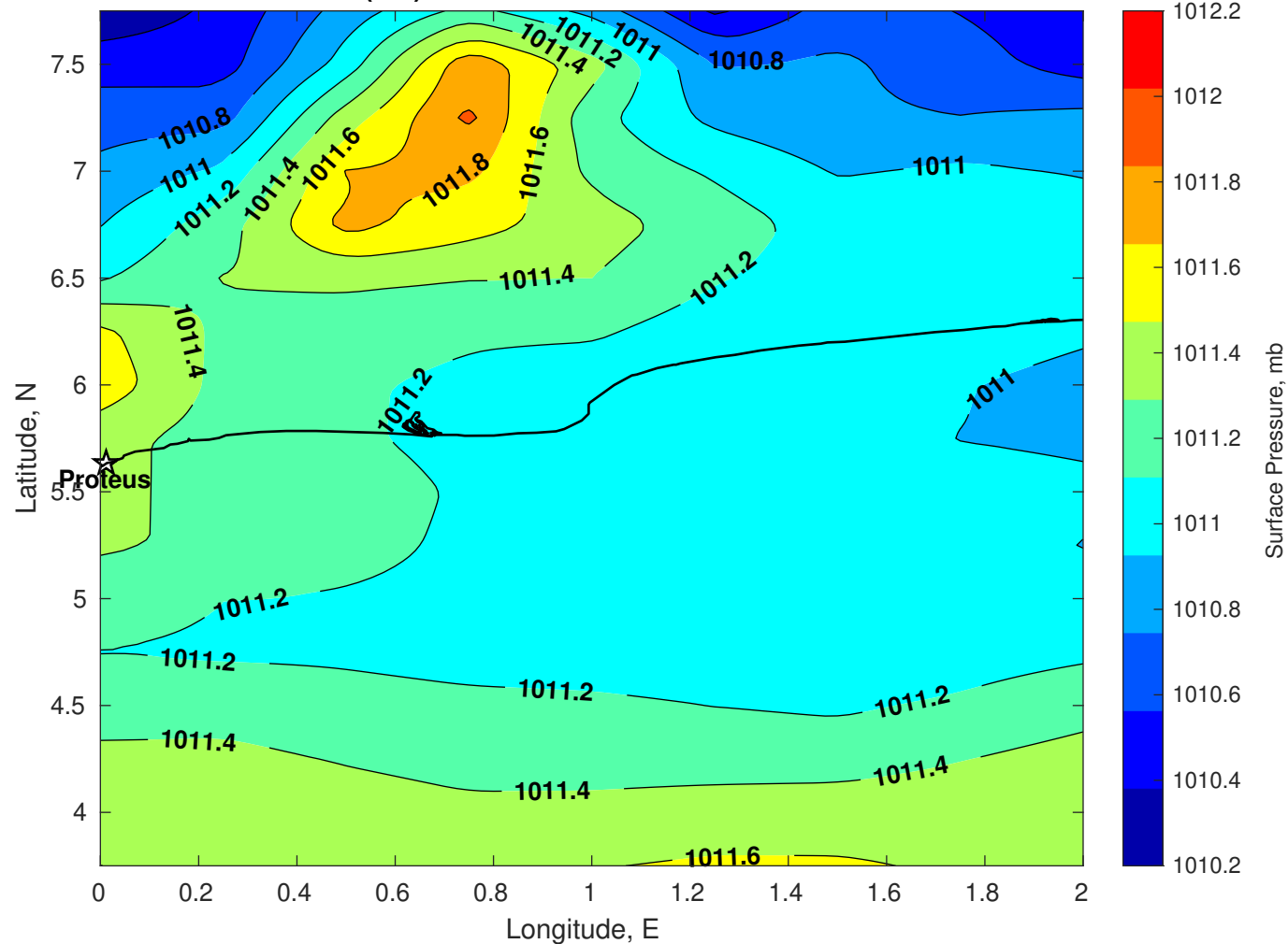
Surface Pressure (mb) for Proteus at 12-Dec-2025 00:00:00
