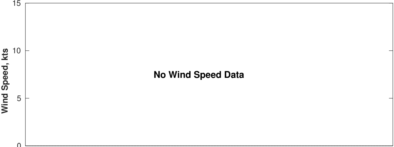
Wind & Wave Forecast for Proteus from 10-Dec-2025 01:00:00 to 26-Dec-2025 01:00:00
