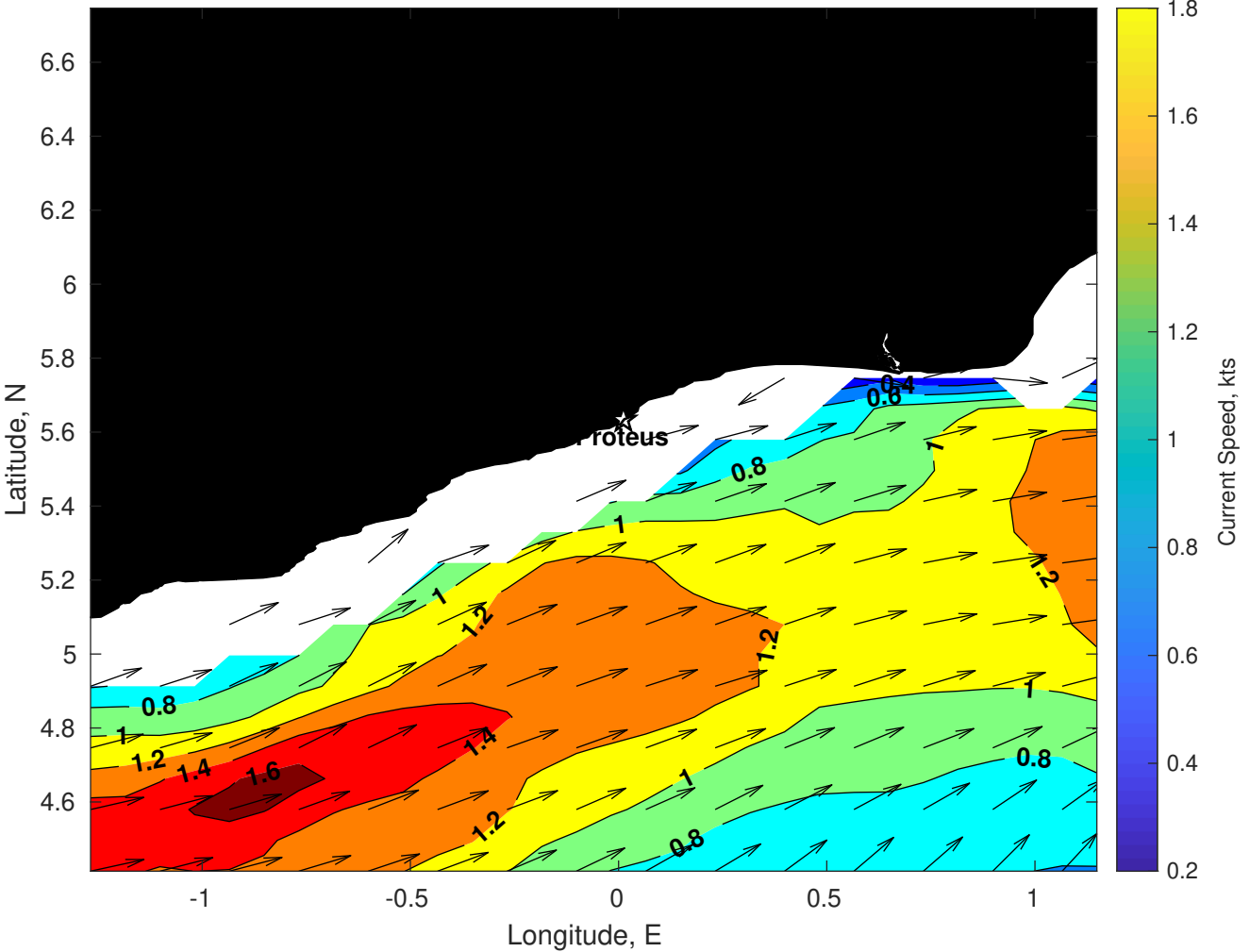
Surface Currents for Proteus at 09-Dec-2025 00:00:00
