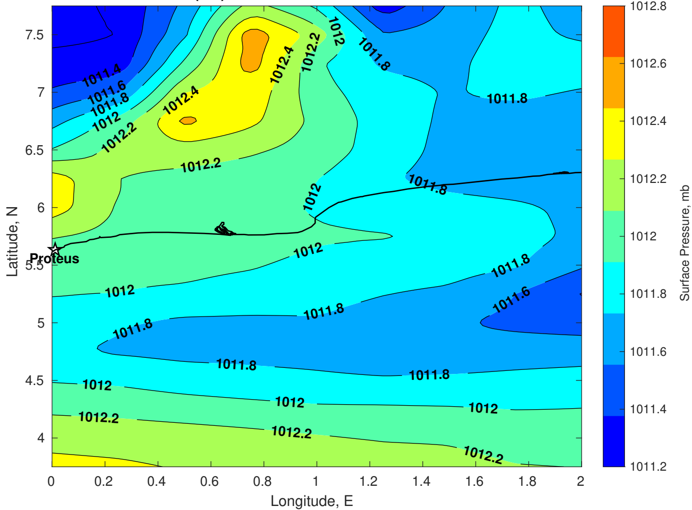
Surface Pressure (mb) for Proteus at 11-Dec-2025 00:00:00
