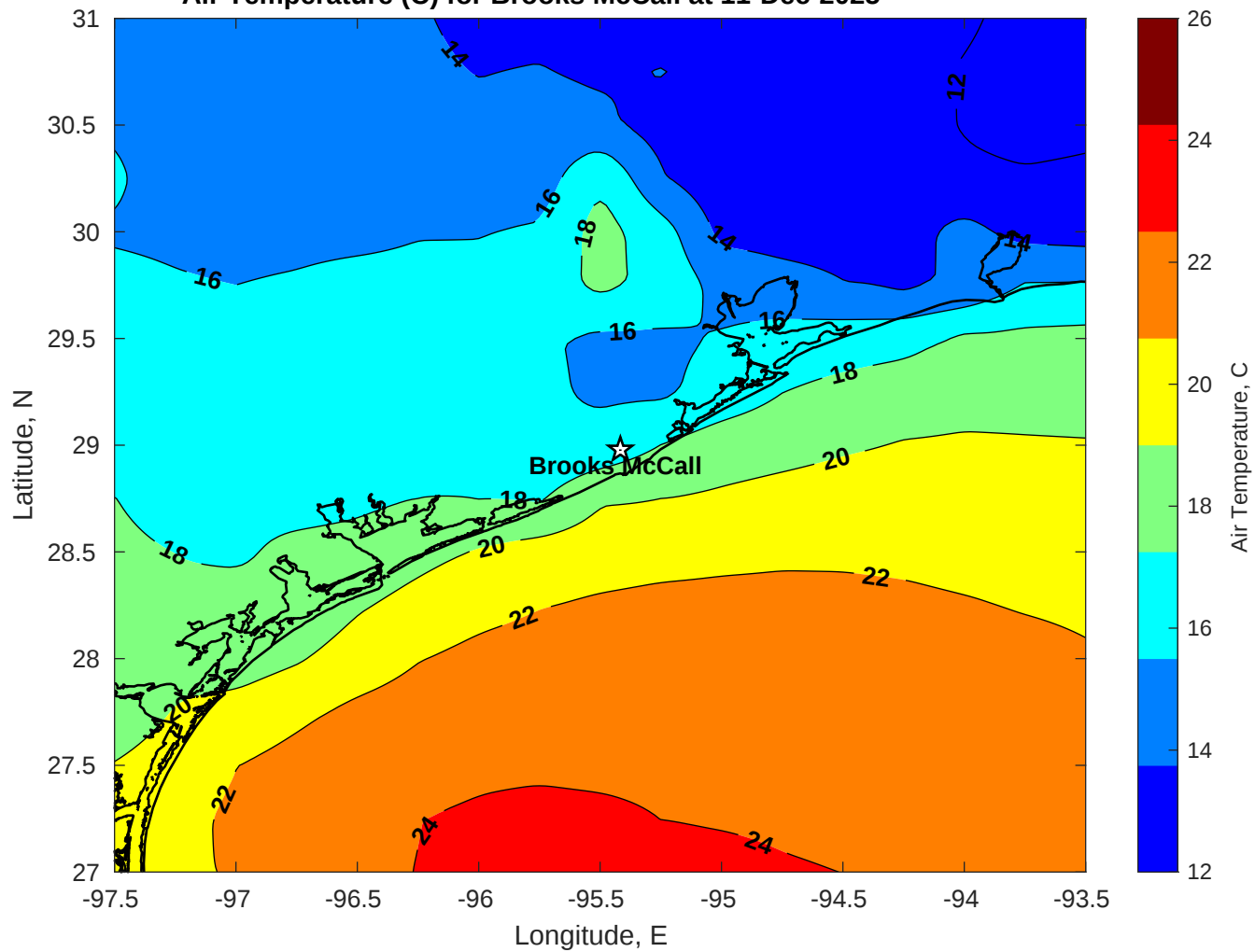
Air Temperature (C) for Brooks McCall at 11-Dec-2025
