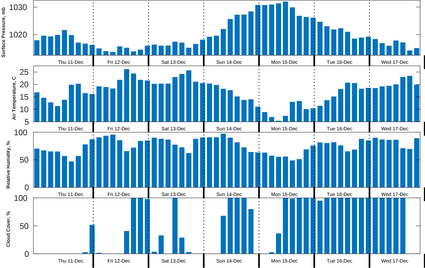
Met Forecast for Brooks McCall from 11-Dec-2025 00:00:00 to 18-Dec-2025 00:00:00
