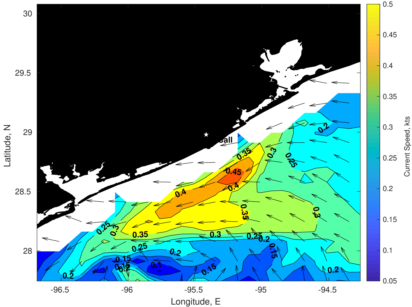
Surface Currents for Brooks McCall at 10-Dec-2025 00:00:00
