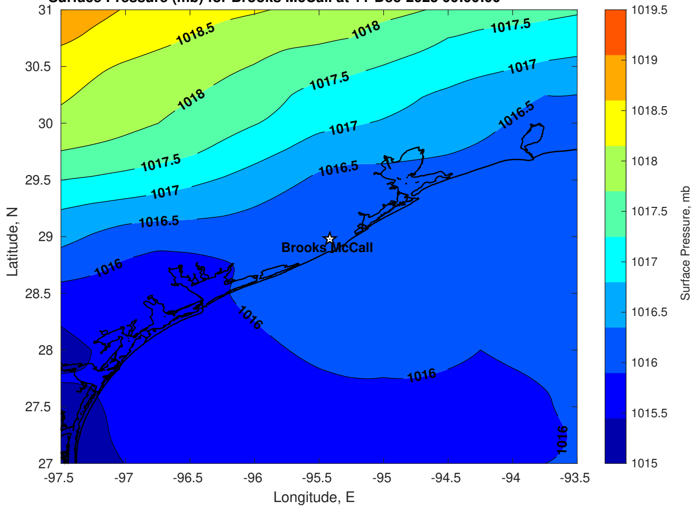
Surface Pressure (mb) for Brooks McCall at 11-Dec-2025 00:00:00
